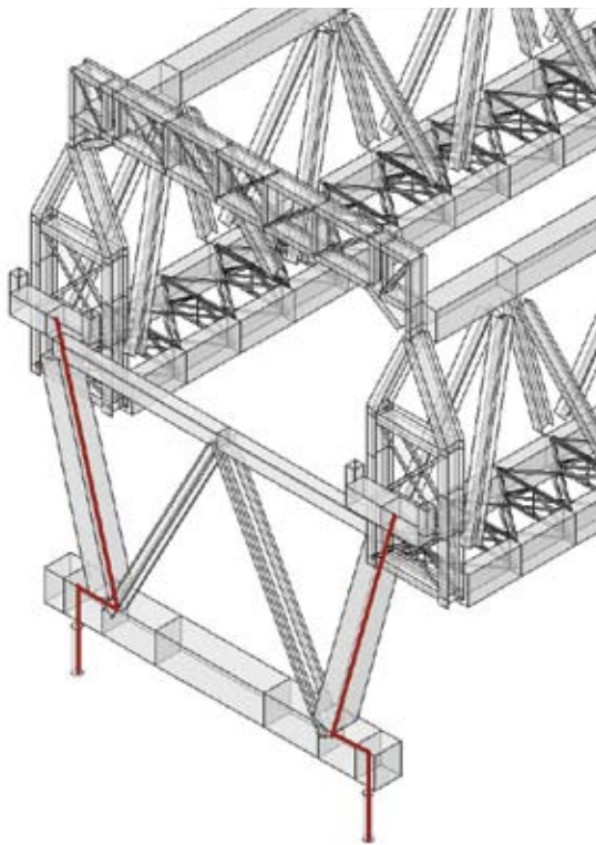
Figure 17. This figure shows a rear portal frame with shifting support pistons.
