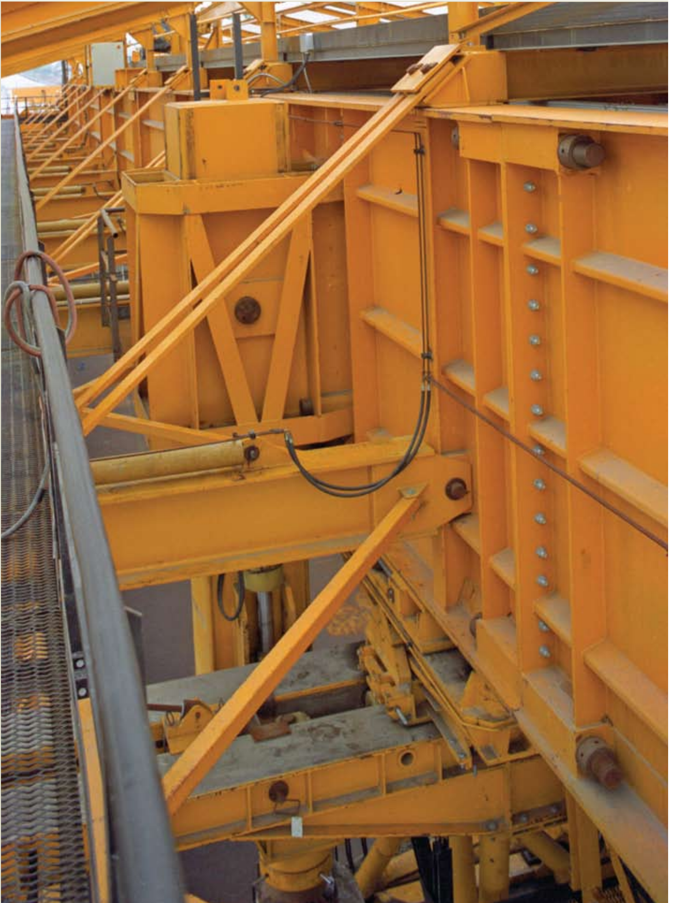
Figure 15. This shows the main structural node of an overhead gantry.
