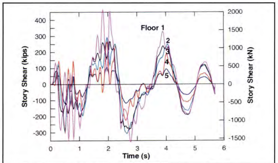
Fig. 11. Time-history of wall direction story shear force response to 1.5xZone 4 excitation.
