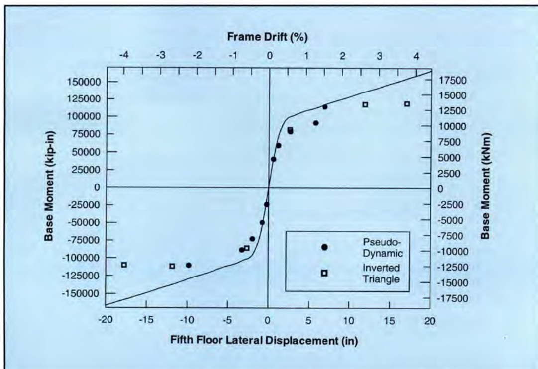
Fig. 30. Comparison of predicted and observed frame direction moment-displacement envelope response.
