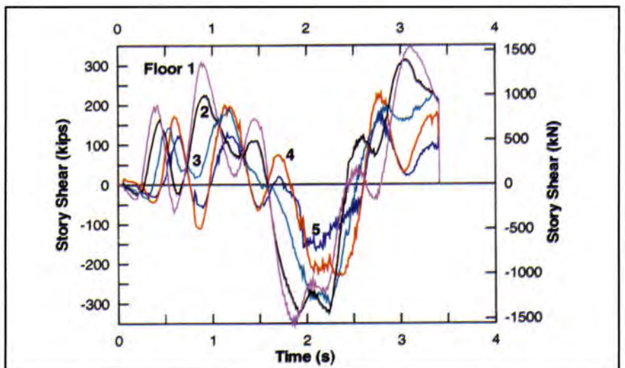
Fig. 21 Time-history of frame direction story shear force response to Zone 4 excitation.
