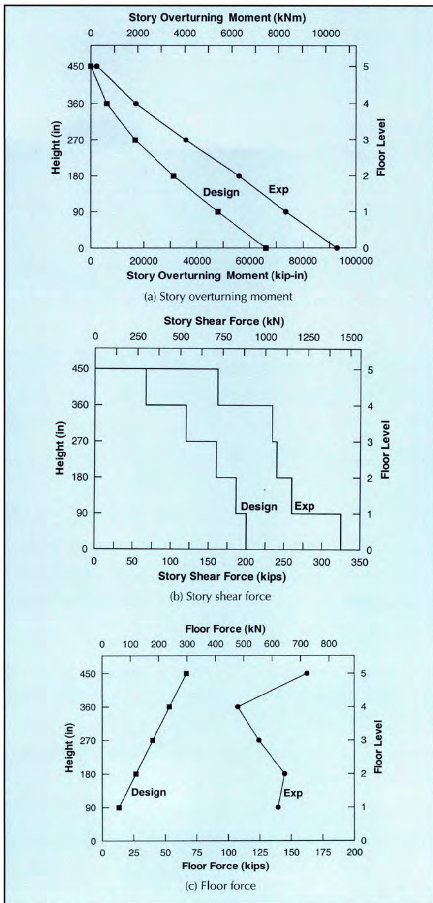
Fig. 14. Comparison of design and experiment force envelopes at design level (Zone 4) excitation.
