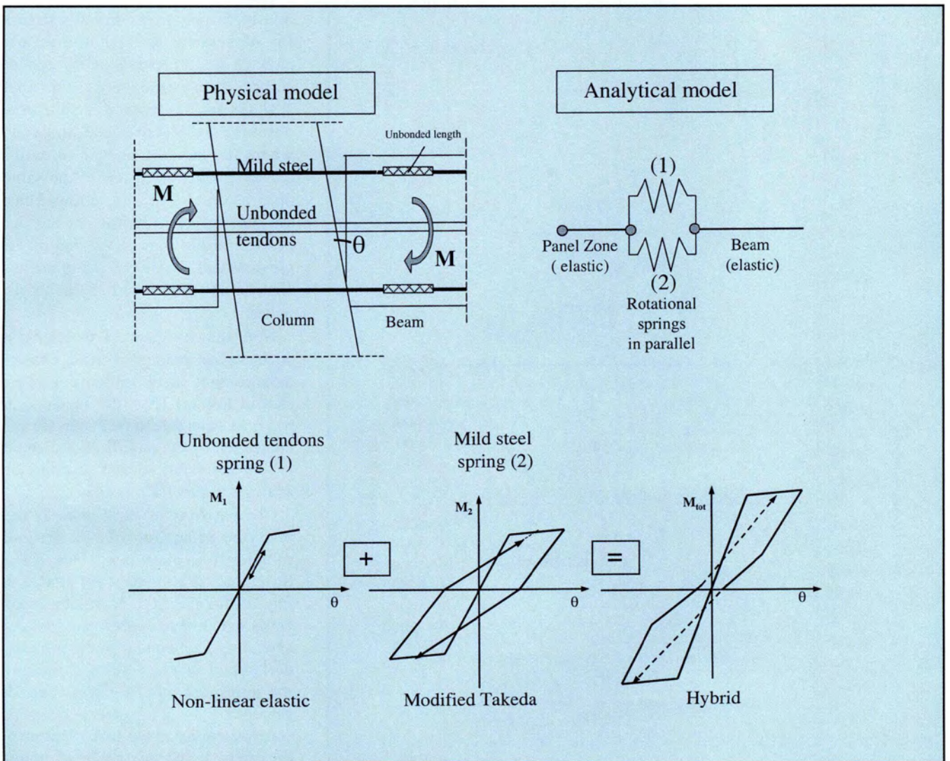
Fig. 28. Analytical model for hybrid prestressed frame connection.
