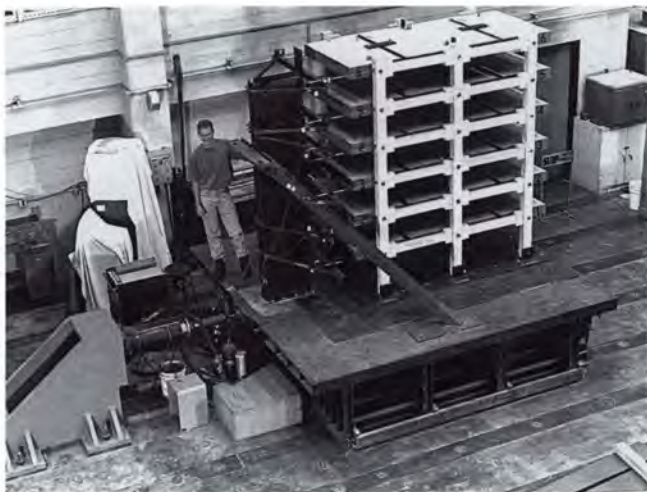
(a) Test structure on earthquake simulator
