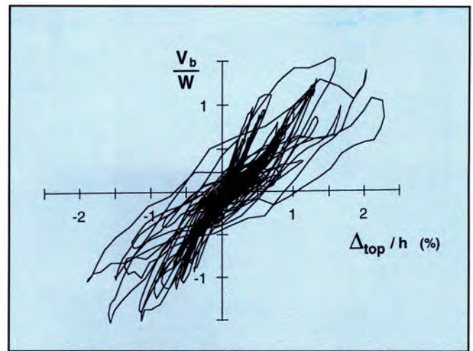
(c) Base shear vs. lateral drift for all test runs
