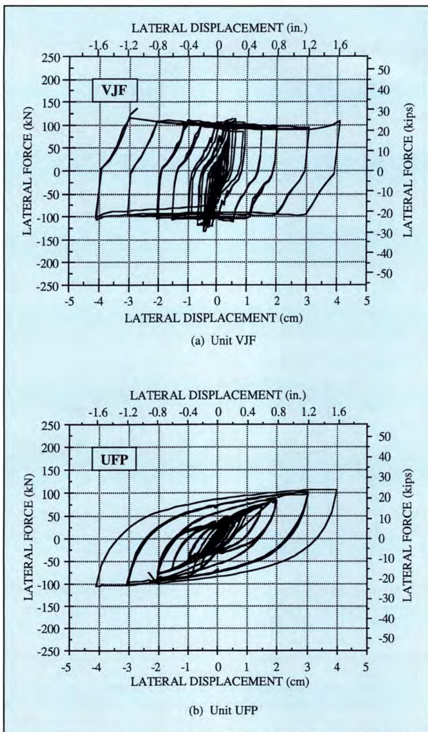
Fig. 9. Load-displacement response for Connections VJF and UFP tested at NIST.
