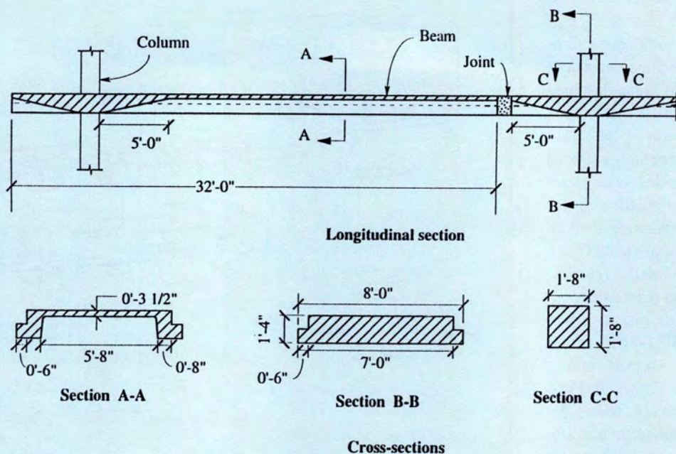
(a) Framing System
