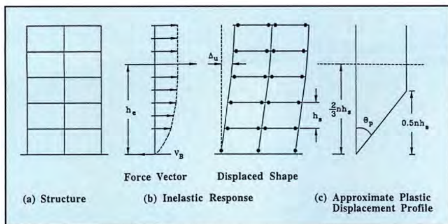
Fig. 18. Maximum response of a frame building.
