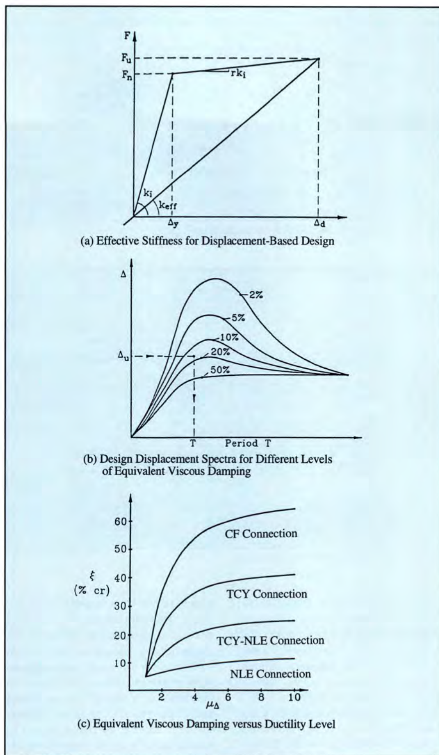
Fig. 17. Elements of displacement-based design procedure.
