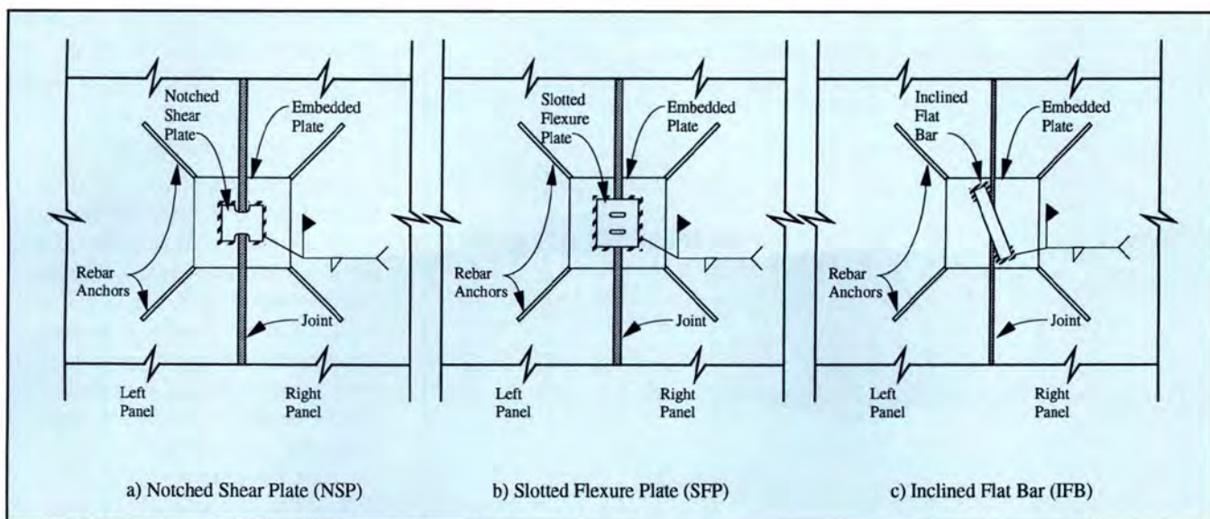
Fig. 7. Welded loose plate connections tested at NIST.
