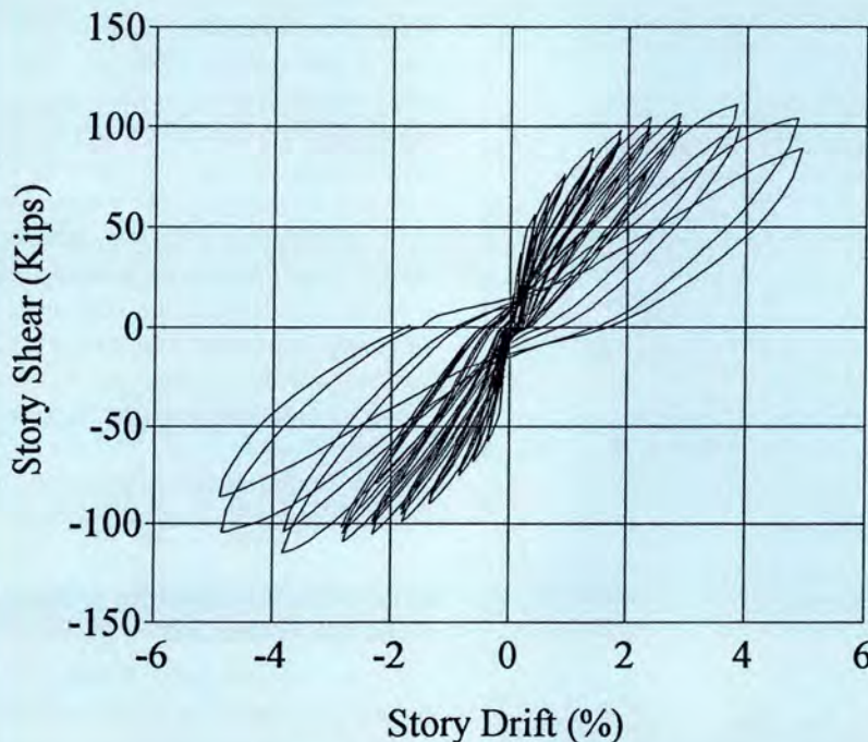
(b) Story Shear – Drift Response
