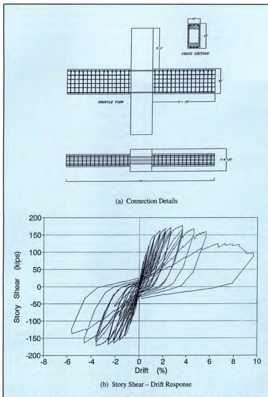
Fig. 3. Unit UMn-TCY tension/compression yield subassembly (University of Minnesota).
