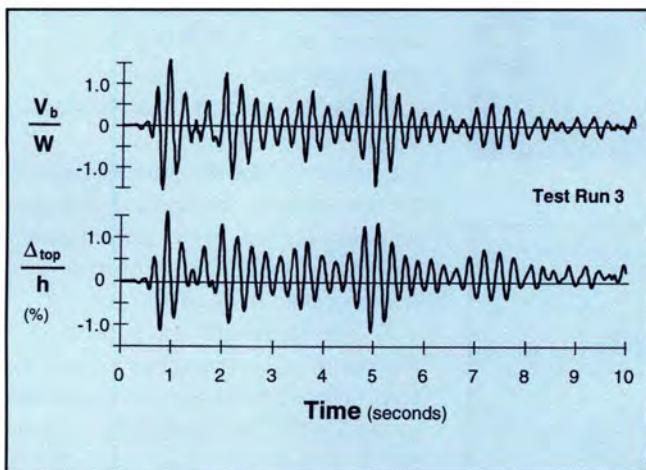
(b) Histories of base shear and lateral drift
