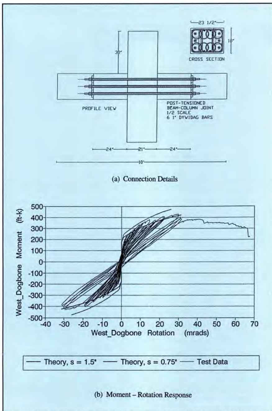
Fig. 2. Unit UMn-PTB elastic non-linear subassembly (University of Minnesota).
