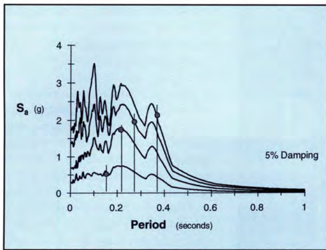
(a) Spectral response curves for Test Runs 1-4
