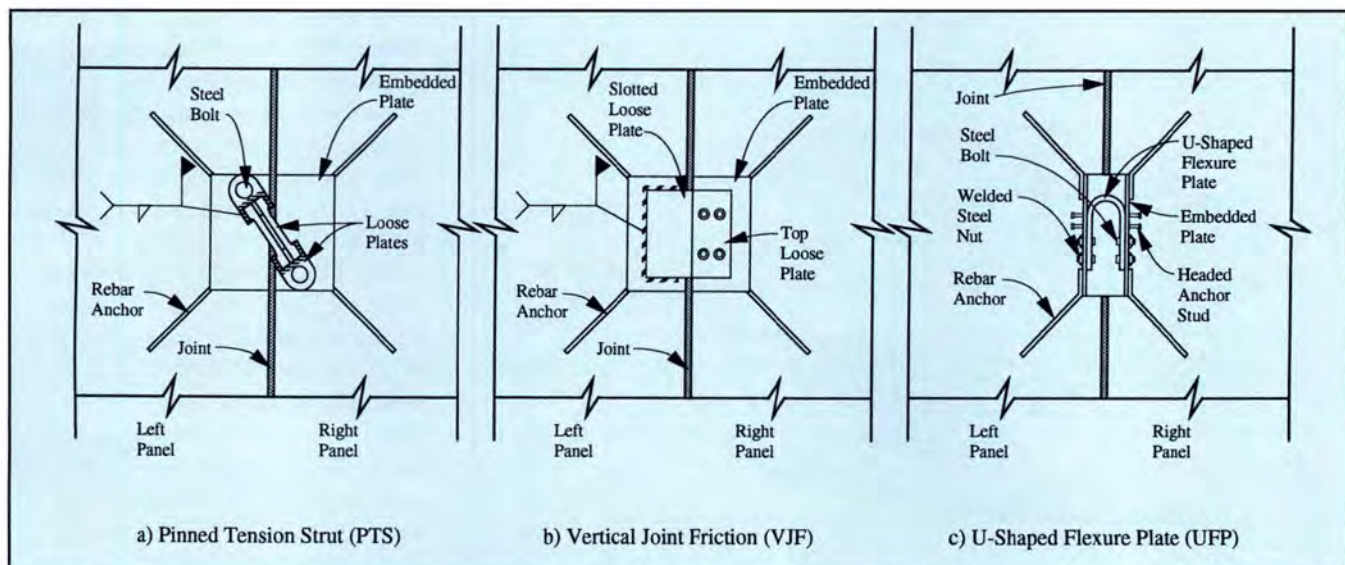
Fig. 8. Bolted ductile connections tested at NIST.
