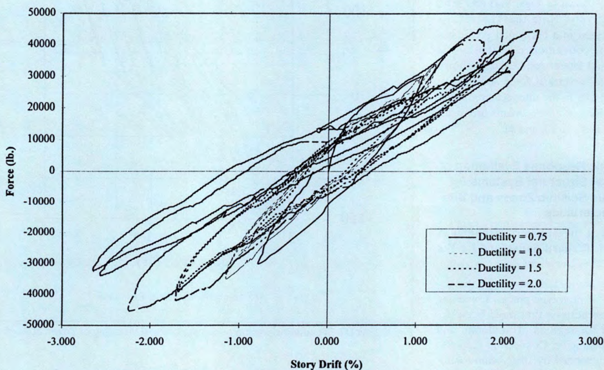
(b) Story Shear - Drift Response
