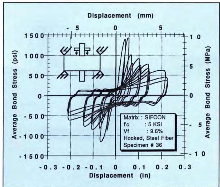
Fig. 14. Bond stress-slip response for a reinforcing bar in SIFCON concrete (University of Michigan).
