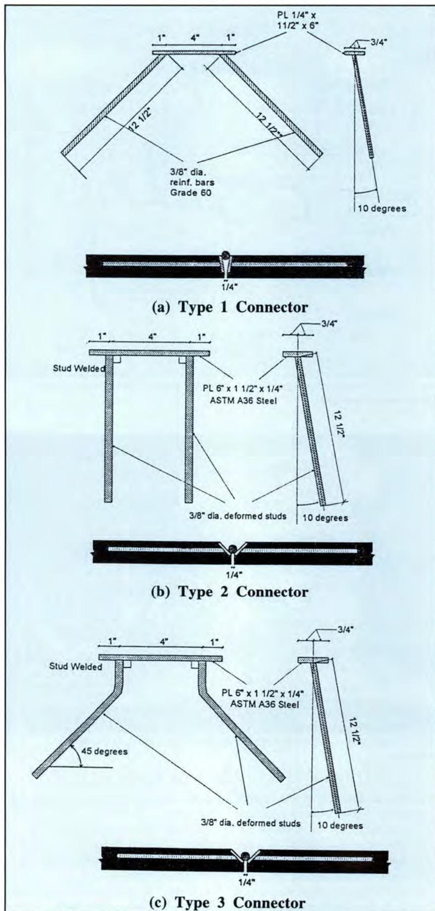
Fig. 16. Flange connectors for double-tee units (University of Wisconsin-Madison).
