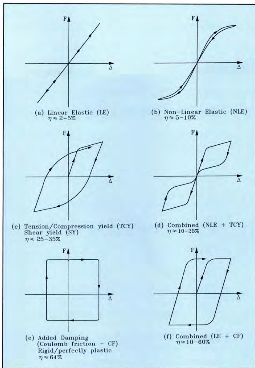
Fig. 1. Hysteretic characteristics for generic PRESSS connection systems ( \eta = equivalent viscous damping).
