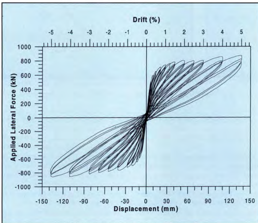
(b) Lateral force-displacement response
