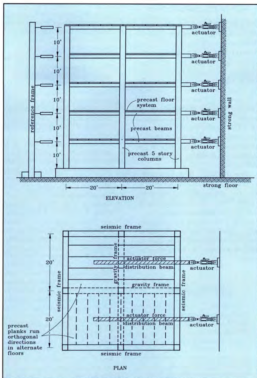
Fig. 20. Eight-tenths full-size precast frame super-assemblage.
