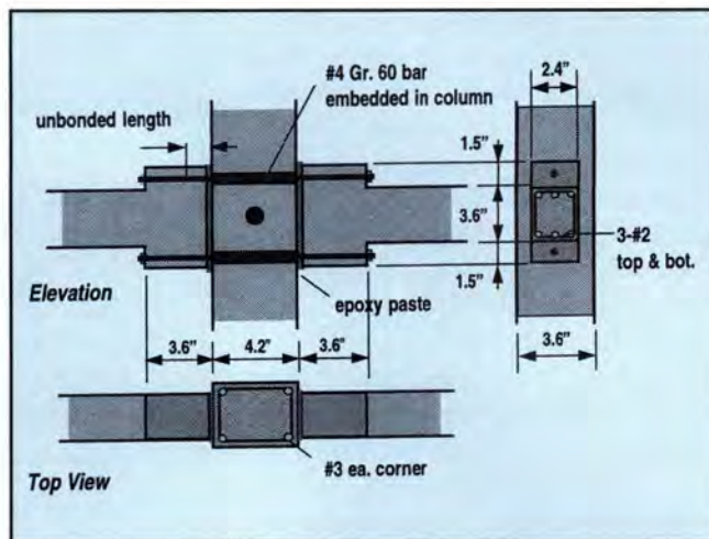
(c) Detail of dog-bone connection
