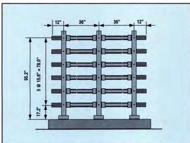
(b) Dimensions of test structure
