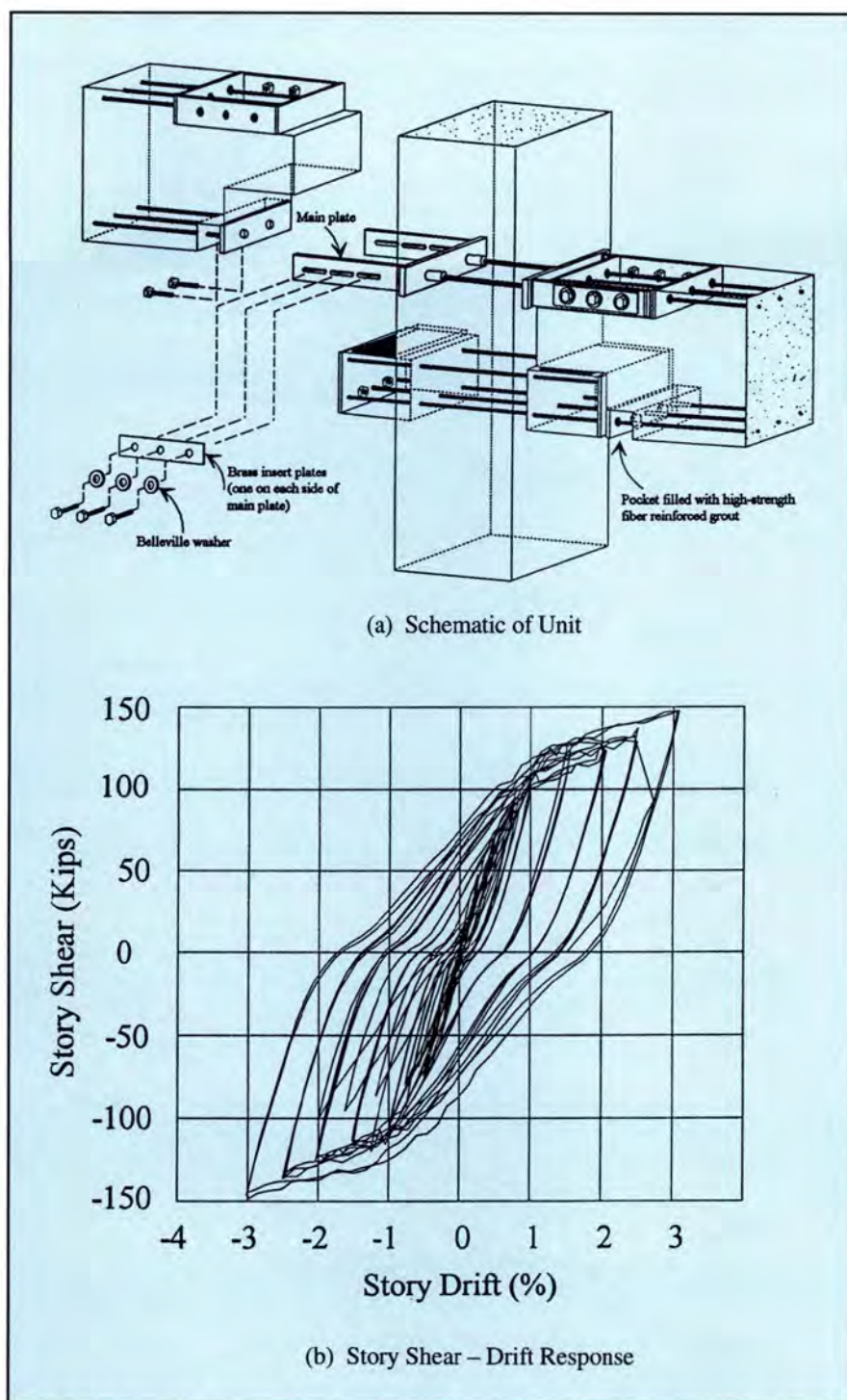
Fig. 5. Unit UT-FR added-damping subassembly (University of Texas at Austin).
