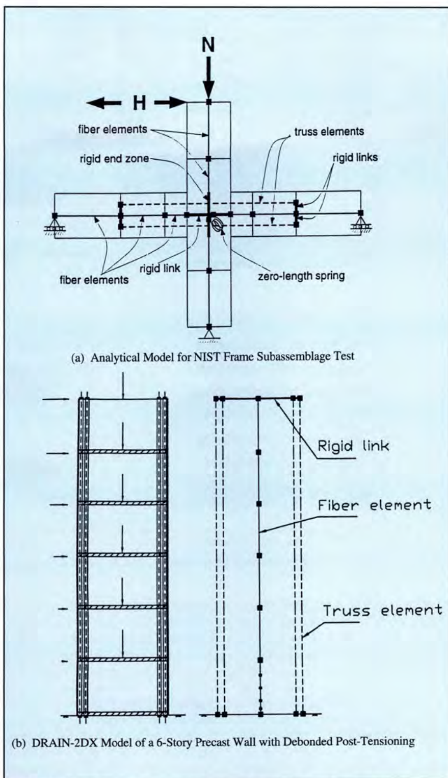
Fig. 10. Analytical models for precast frames and panel structures utilized in Lehigh University studies.
