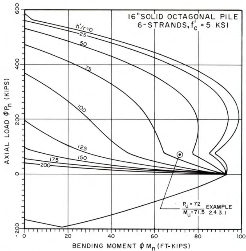
Fig. 2.5. Interaction curve for 16 in. (406 mm) octagonal pile.
