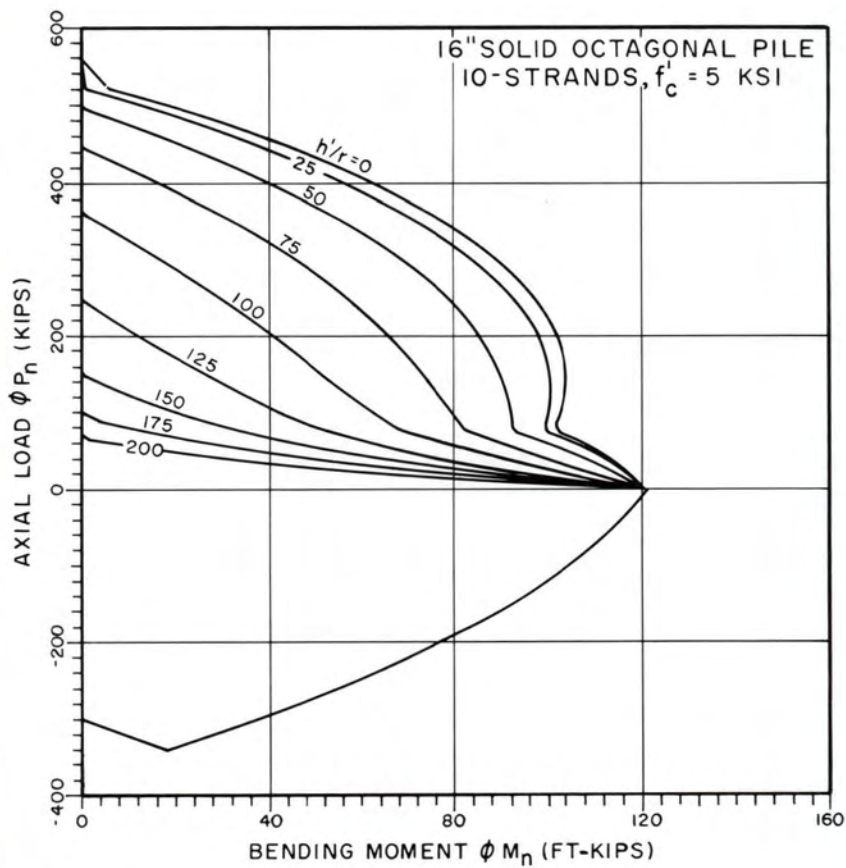
Fig. 2.6. Interaction curve for 16 in. (406 mm) octagonal pile.
