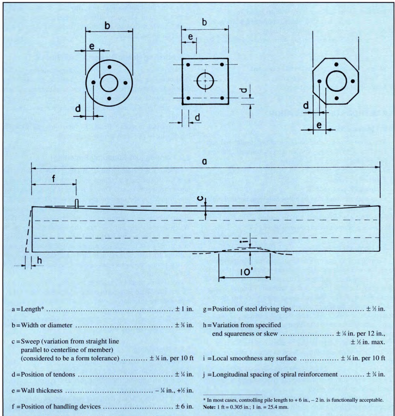
Fig. 4.2. Prestressed concrete pile production tolerances.
