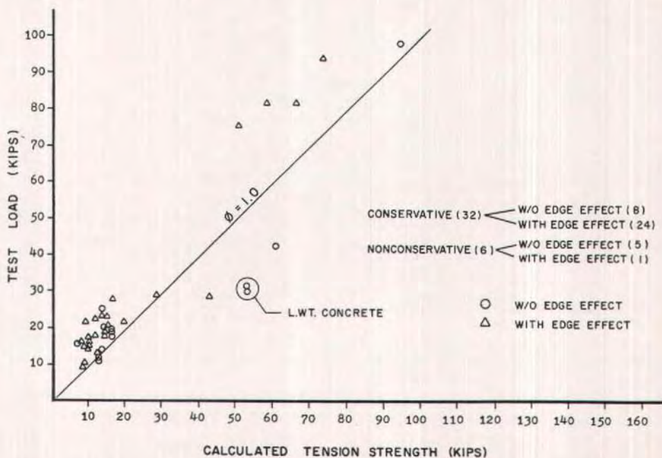
Fig. 11. Calculated tension strength [Eq. (12)] versus test load.
