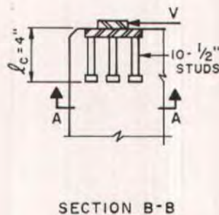
Fig. 20. Cross section of stud connection for Example 1.
