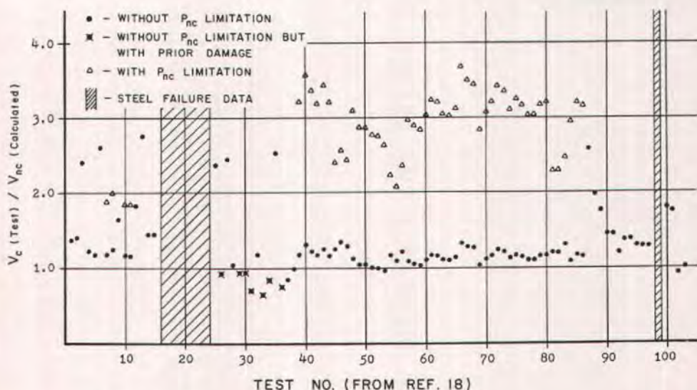
Fig. 17. Effect of pull-out strength limitation on shear strength.
