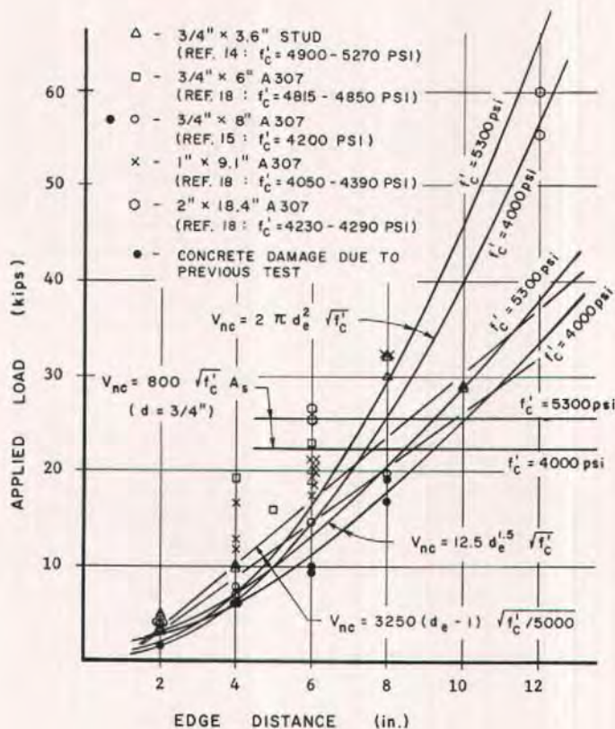
Fig. 16. Shear on studs located close to edge.
