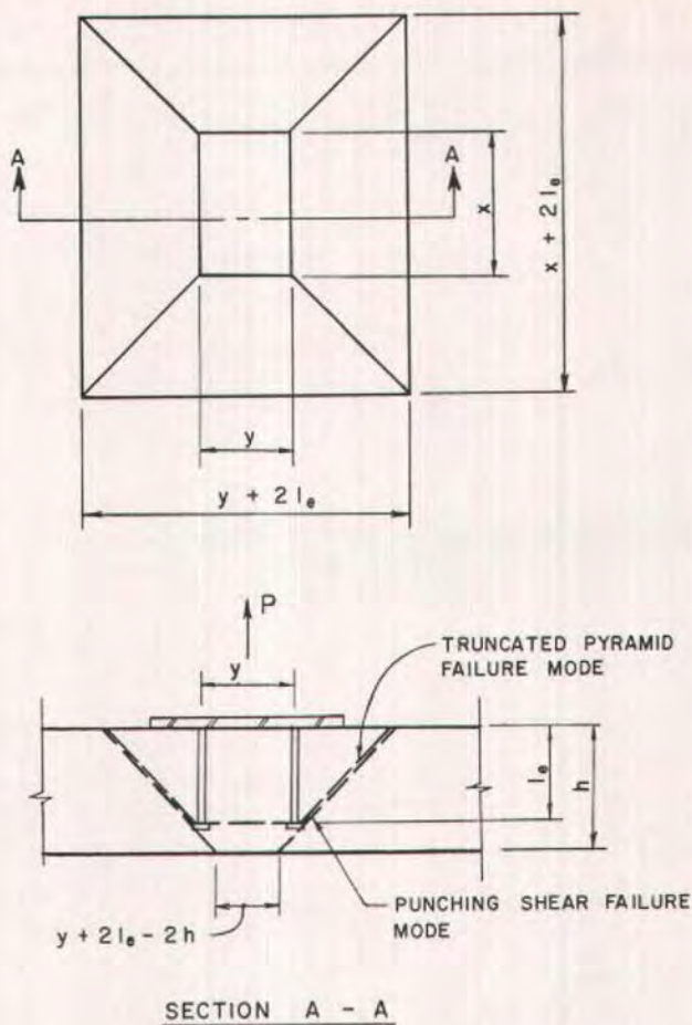
Fig. 14. Truncated pyramid and punching shear failures.
