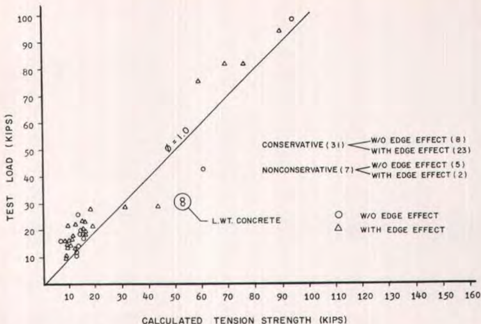
Fig. 9. Calculated tension strength [Eq. (10)] versus test load.
