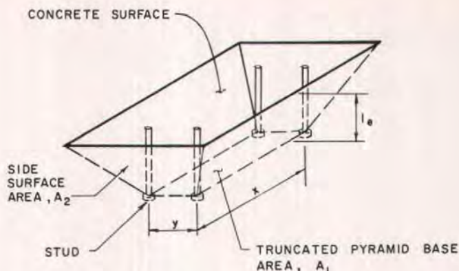
Fig. 12. Truncated pyramid failure for a stud group in tension.
