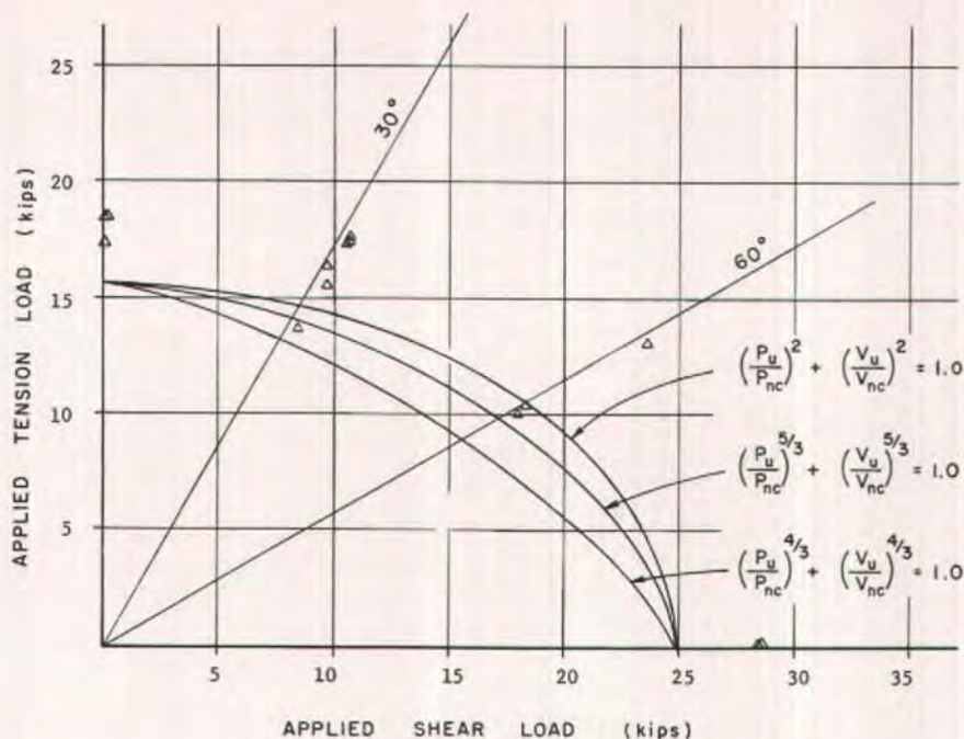
Fig. 19. Studs under combined shear and tension (experimental data from Ref. 14).
