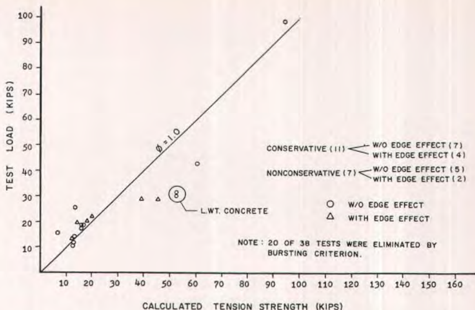
Fig. 6. Calculated tension strength (ACI 349 12 ) versus test load.
