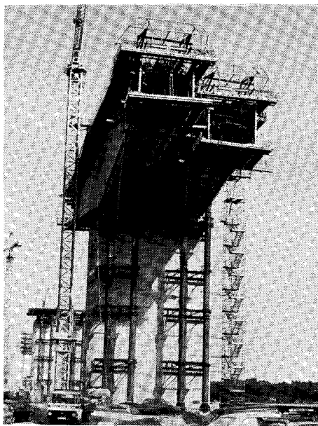
Fig. 9. Orwell Bridge, United Kingdom.
