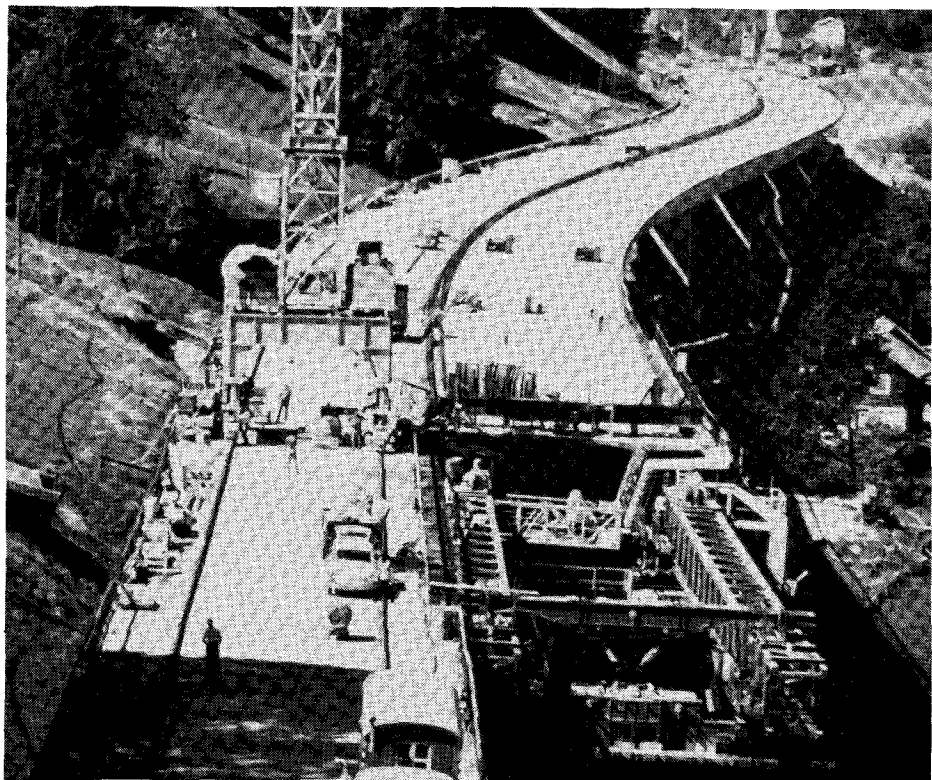
Fig. 3. Beckenried Viaduct, Switzerland.
