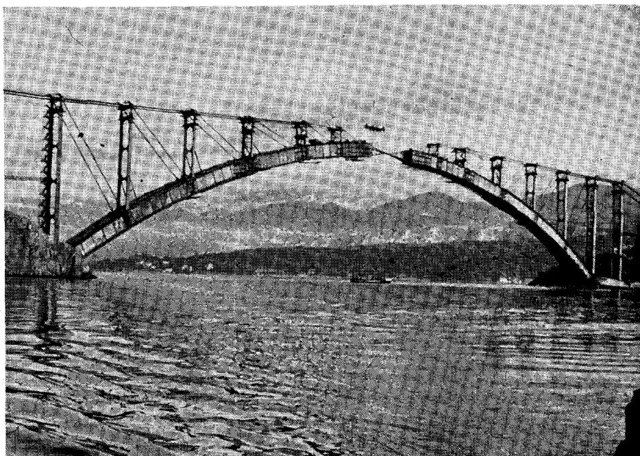
Fig. 24. Krk Bridge, Yugoslavia.
