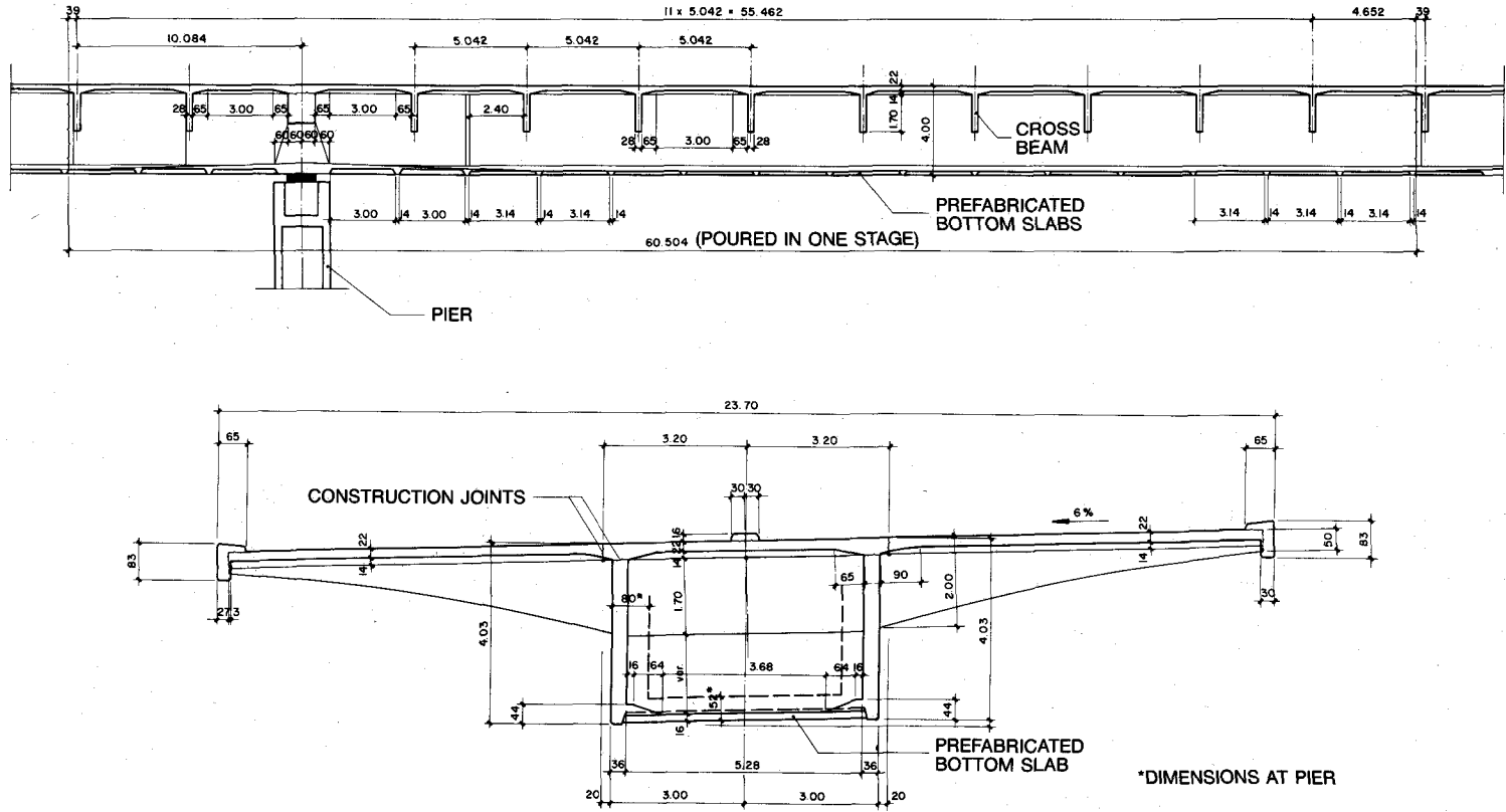
Fig. 5. Gruyère Viaduct, Switzerland. Longitudinal section (top) and cross section at midspan (bottom).
