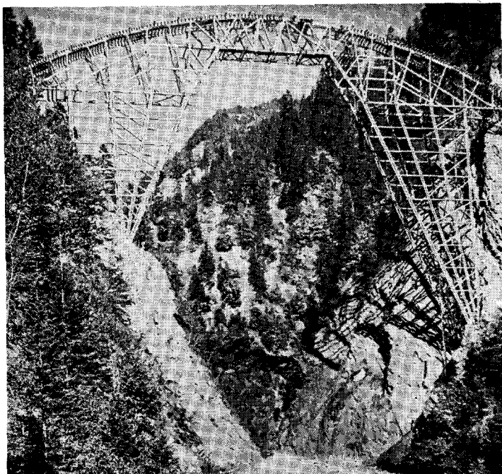
Fig. 23. Salginatobelbridge, Switzerland. Scaffolding.
