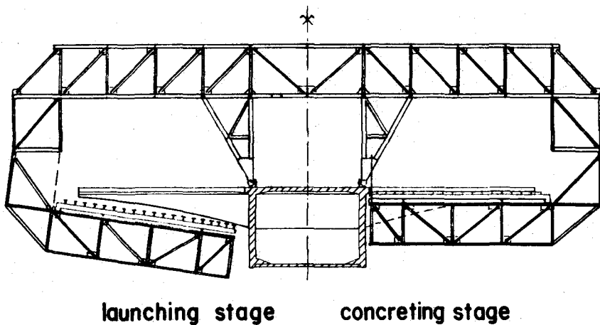
Fig. 8. Gruyère Viaduct, Switzerland. Formwork carriage.
