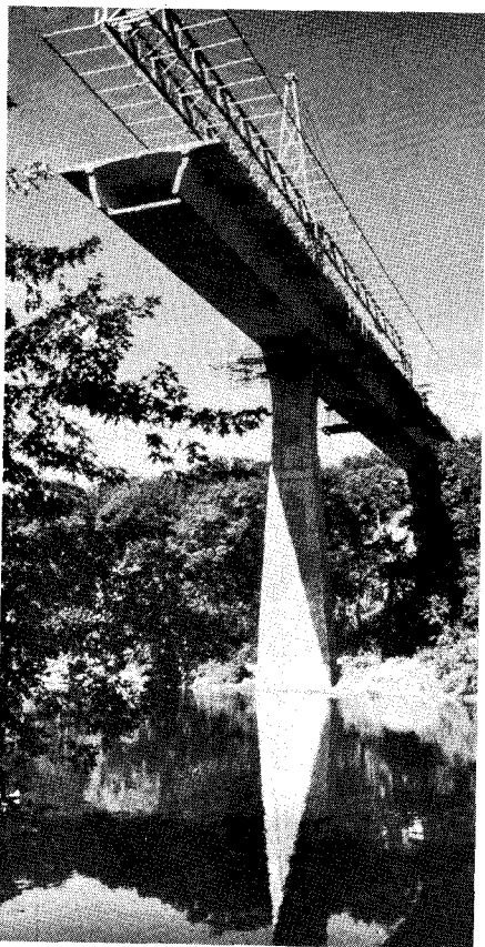
Fig. 8a. Kishwaukee River Bridge near Rockford, Illinois.
