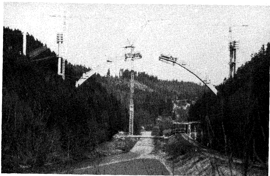
Fig. 33. Arch just before closure section of Talbrücke Rottweill-Neckarburg Bridge southwest of Stuttgart, West Germany. (Courtesy: W. Zellner.)
