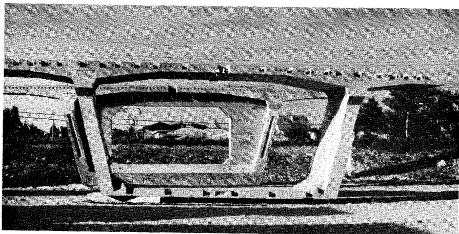
Fig. 8b. Precast segments for Kishwaukee River Bridge near Rockford, Illinois.
