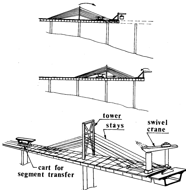
Fig. 10. Progressive placing erection (Reference 7).
