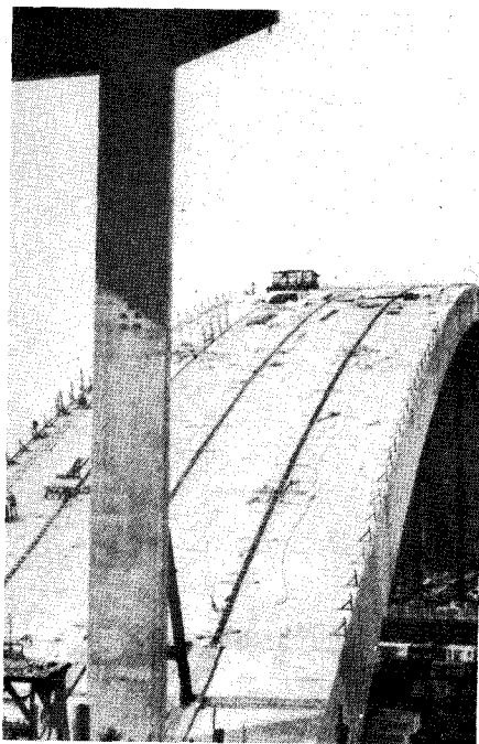
Fig. 32. Completed four arch ribs of Gladesville Arch Bridge, Australia (Reference 14).
