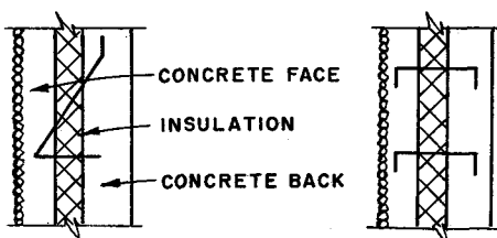
Fig. 5. Ties in sandwich panels.
