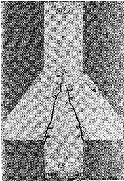
(a) Tension Failure (FT)
