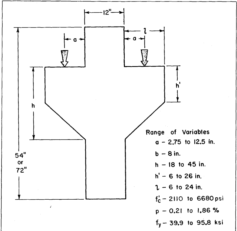
Fig. 5—Corbel Test Specimen
