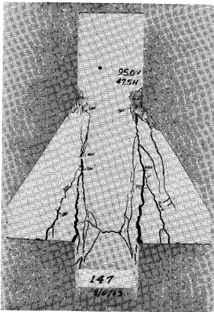
Fig. 20—Flexural Yielding Failure Followed by Crushing of the Concrete (FT), H/V = 1
