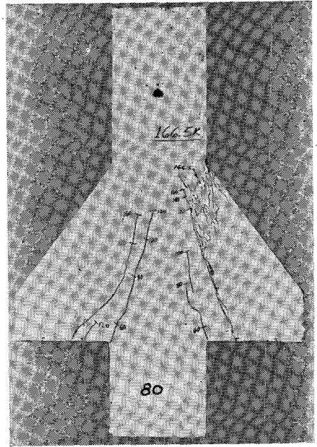
(b) Compression Failure (FC)
