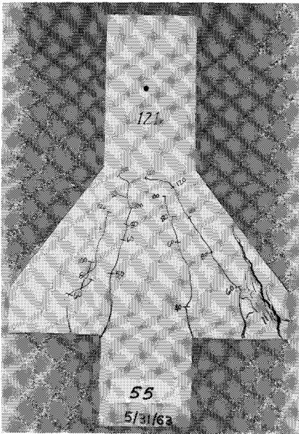
(a) Corbel End Failure (CE)
