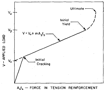
Fig. 17—Idealized Relationship Between Applied Load and Force in Tension Reinforcement
