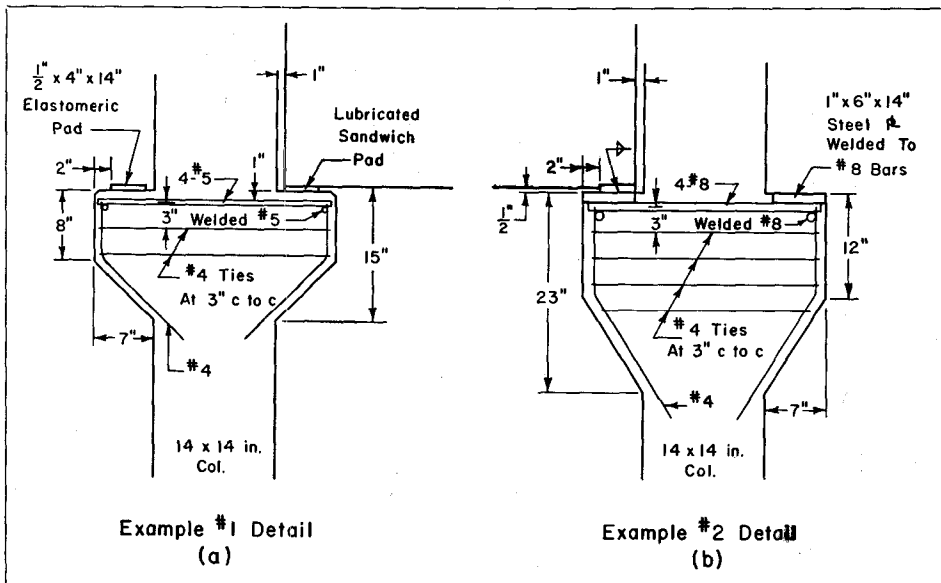
Fig. 4—Corbel Details for Example Problems
