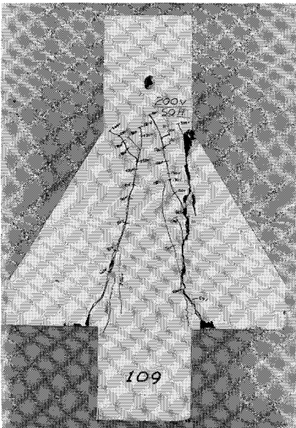
Fig. 21—Shear Failure (S), H/V = 1/2
