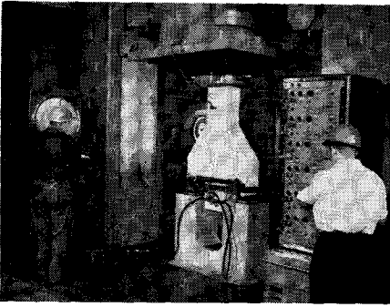
Fig. 10—Test Setup for Combined Horizontal and Vertical Loading, H/V does not equal zero
