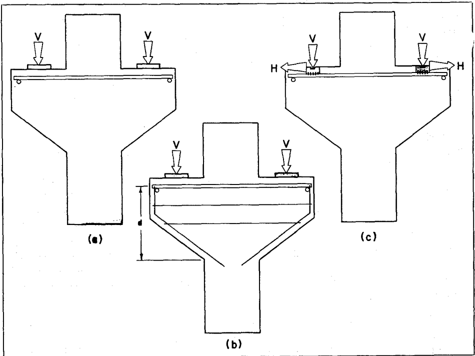
Fig. 6—Reinforcement Details of Test Corbels
