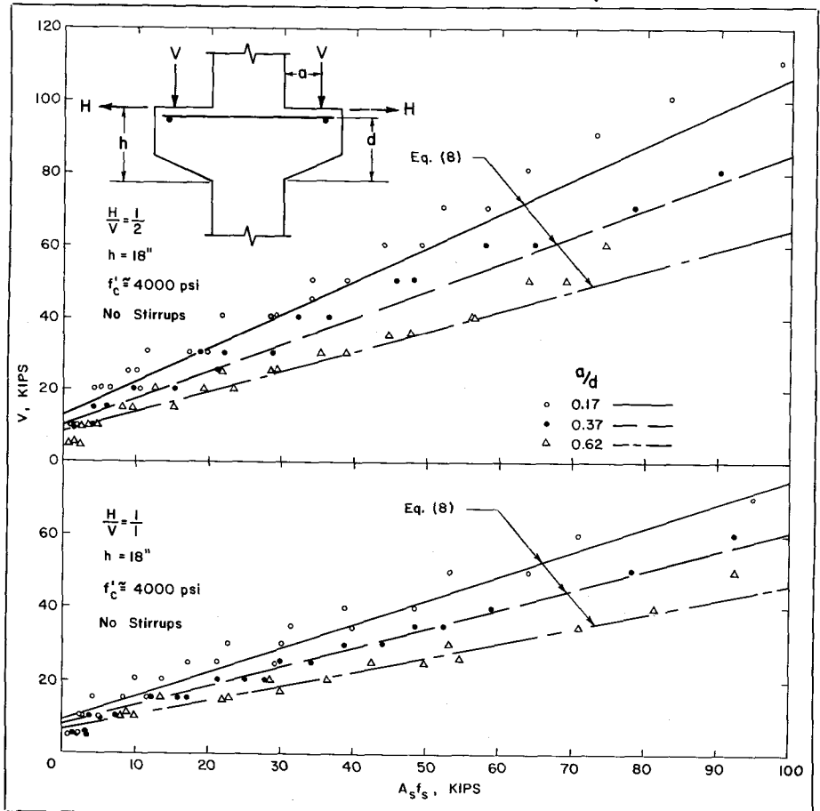
Fig. 19—Relationship Between Applied Load and Tension Steel Force, Combined Vertical and Horizontal Loading
