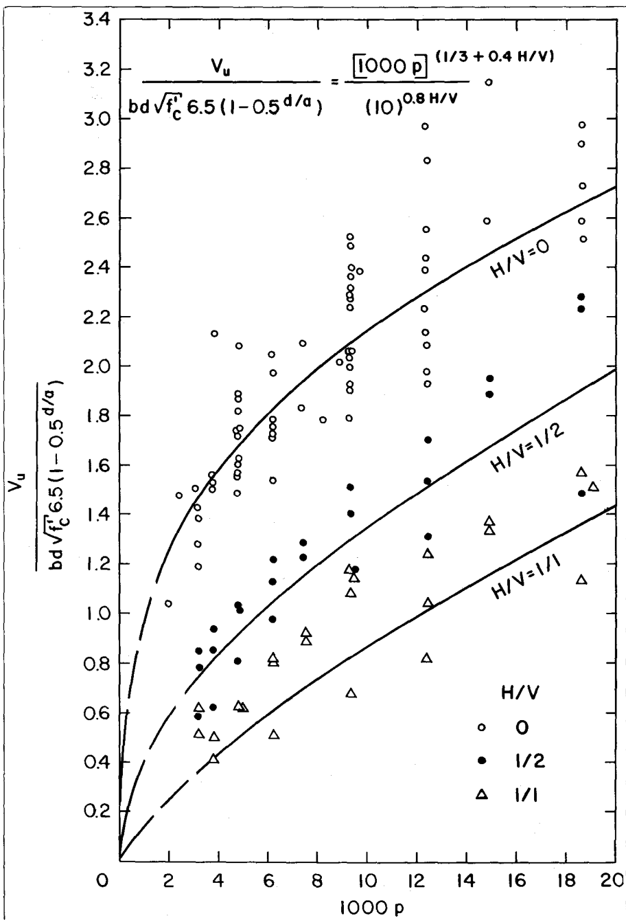
Fig. 18—Ultimate Strength of Corbels
