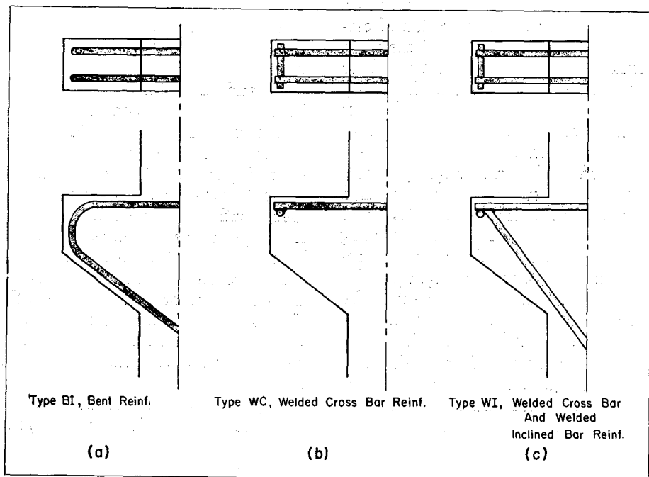
Fig. 7—Detailing of Corbel Reinforcement in Auxiliary Test Series
