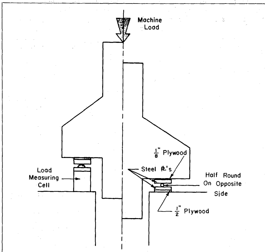
Fig. 8—Vertical Loading of Corbels
