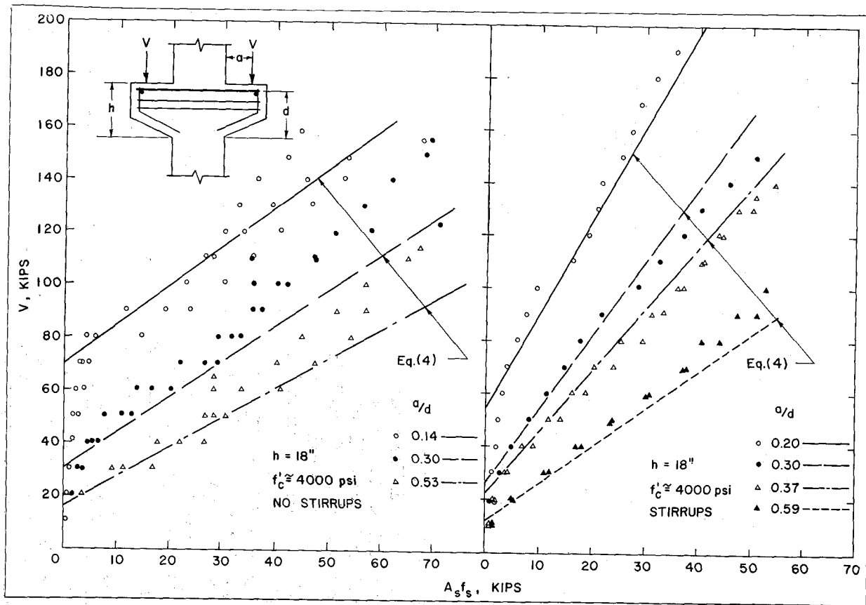
Fig. 12—Relationship Between Applied Load and Tension Steel Force, Vertical Load Only
