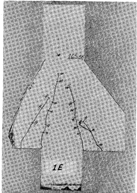
Fig. 11—Conventionally Reinforced Corbel, Type B1, Loaded Near Outer Edge. Failure Plane Follows Bend Radius
