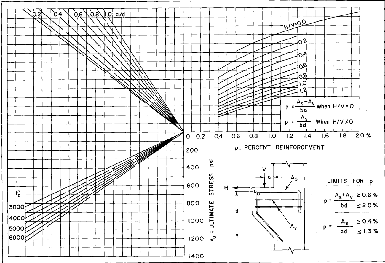
Fig. 3—Design Chart for Ultimate Strength of Corbels
