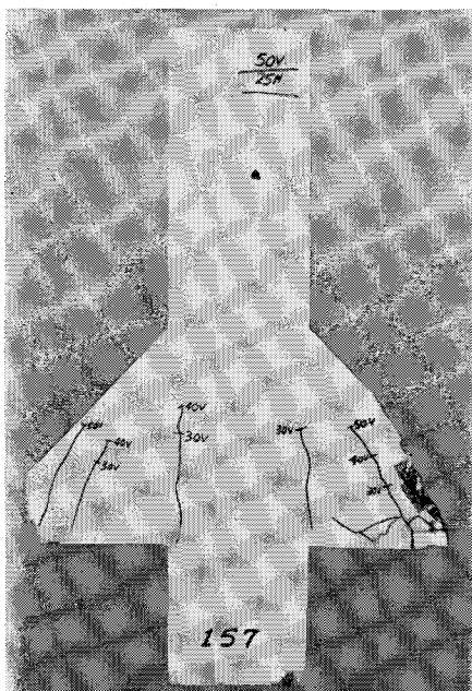
Fig. 22—Corbel End Failure (CE), H/V = 1
