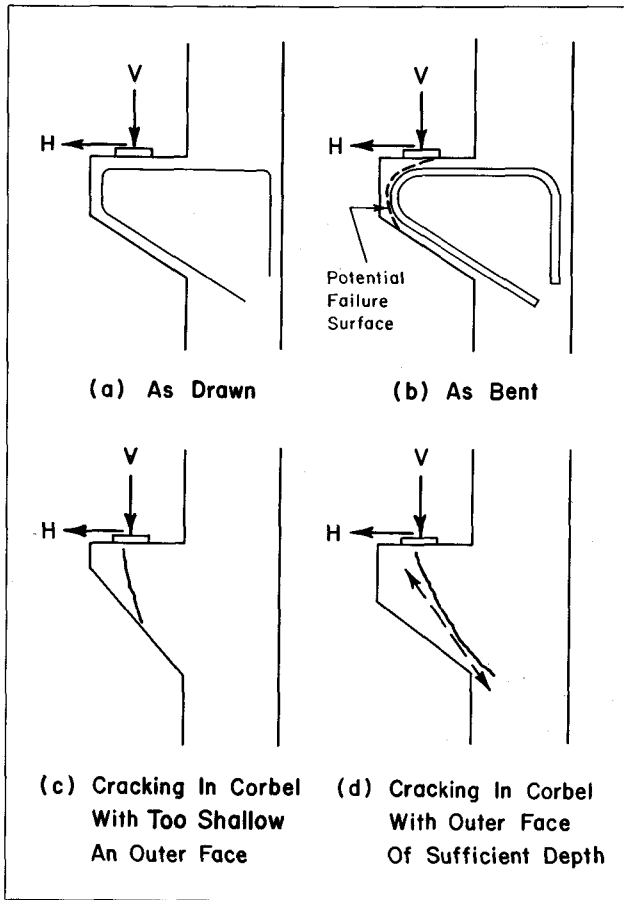
Fig. 2—Corbel Details
