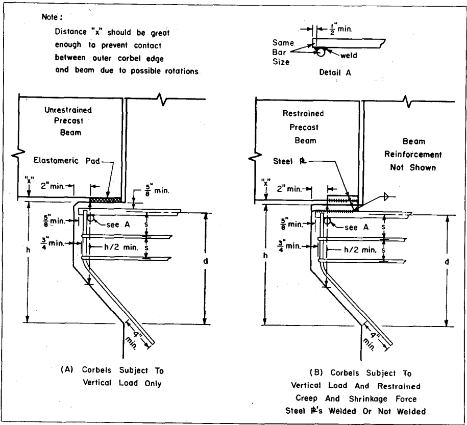
Fig. 1—Recommended Corbel Details
