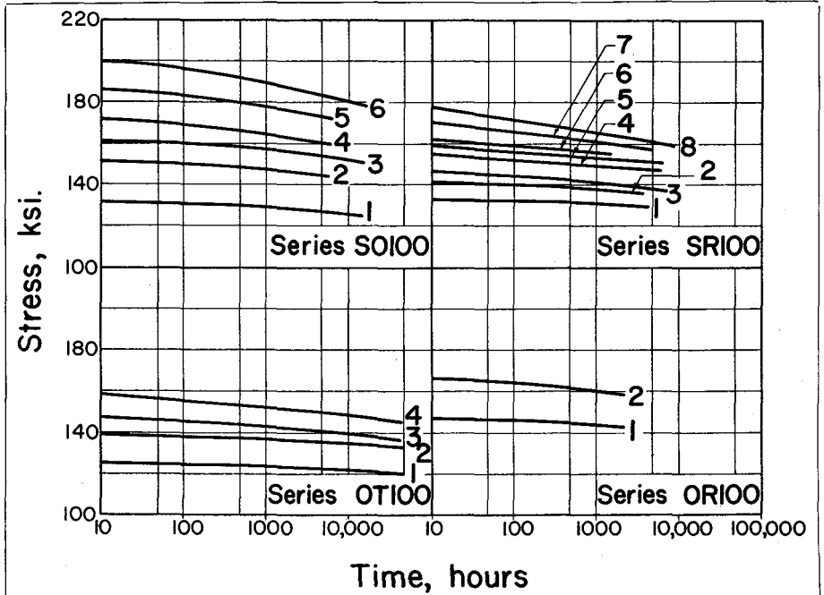
Fig. A.3—Measured Variation of Steel Stress with Time; Series SO100, SR100, OT100, and OR100.
