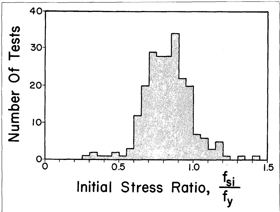
Fig. 2—Frequency Distribution of Initial Stress Ratios.
