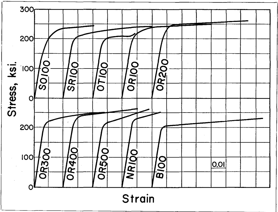
Fig. A.1—Stress-Strain Curves.
