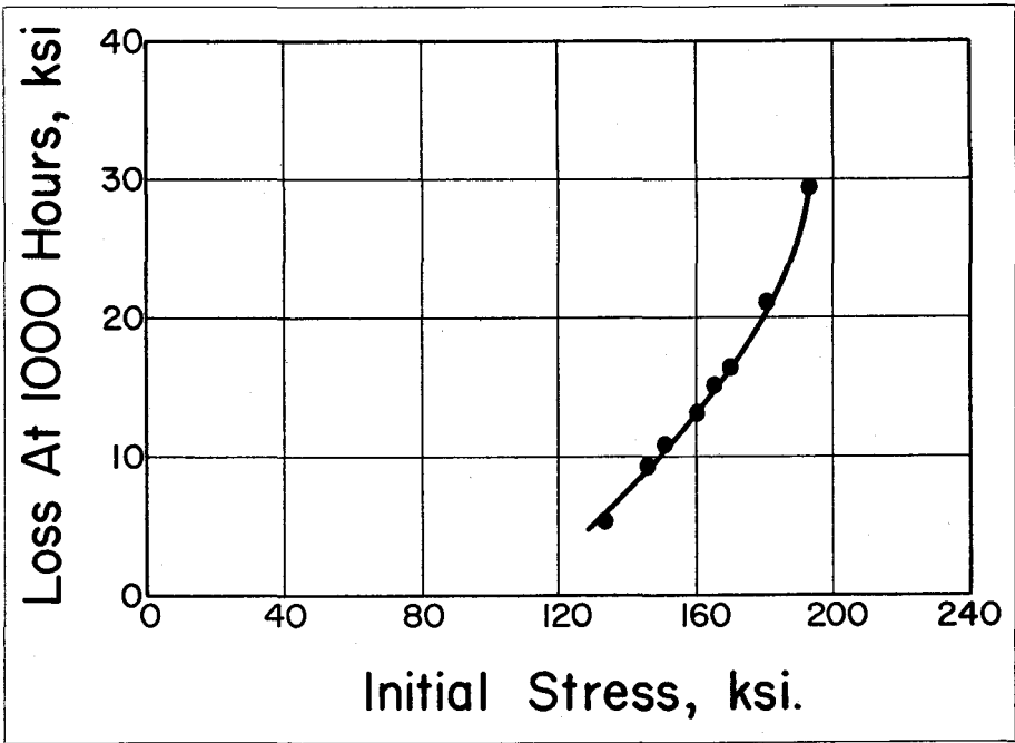
Fig. 3—Effect of Initial Stress Level on Relaxation Loss; Data from Series SR100, Appendix A.
