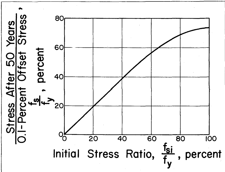
Fig. 9—Comparison of the Remaining Stress After 50 Years Based on Equation 1 with the Initial Stress.
