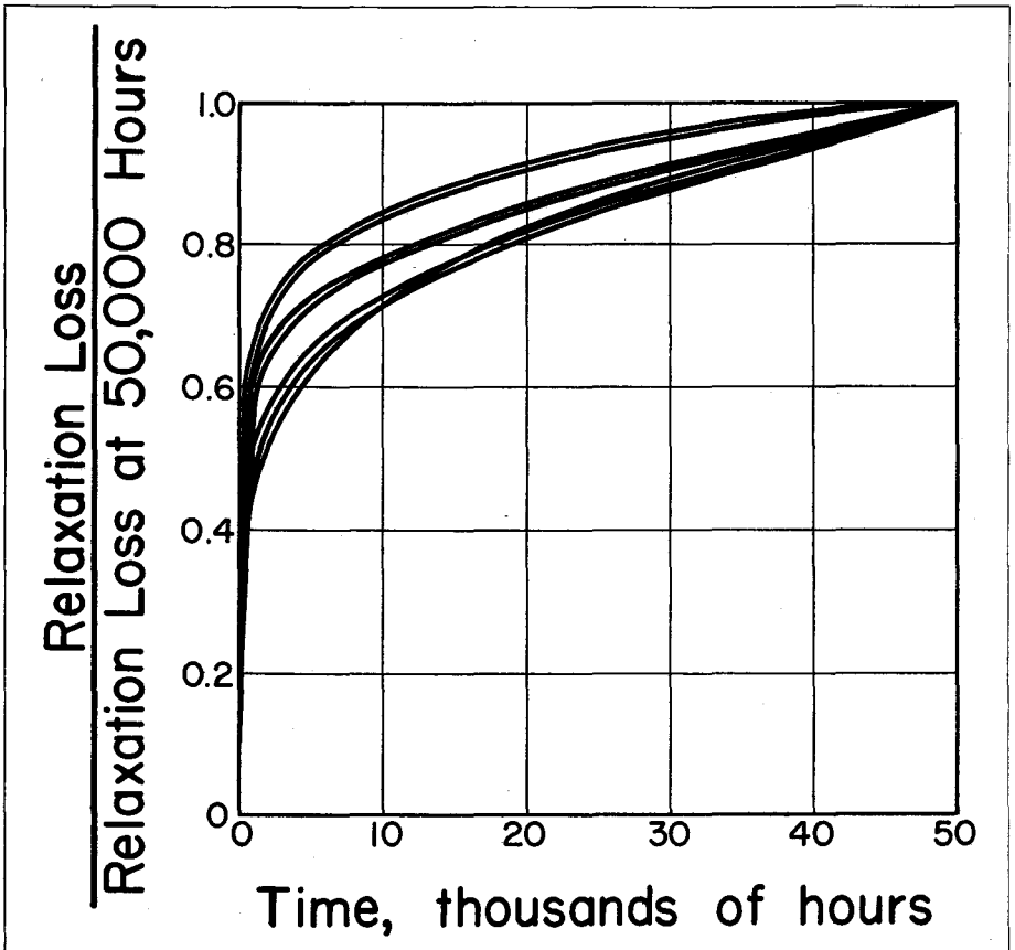
Fig. 5—Rate of Relaxation Loss.
