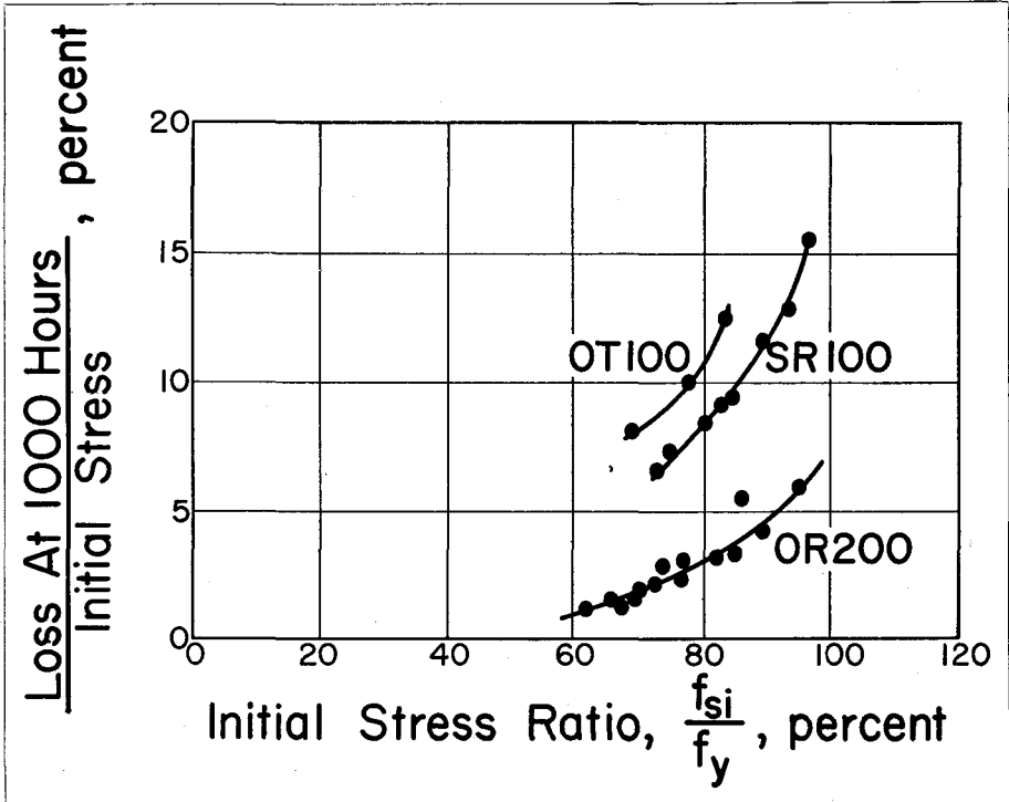
Fig. 4—Effect of Initial Stress Level on Relaxation Loss; Data from Series OT100, SR100, and OR200, Appendix A.
