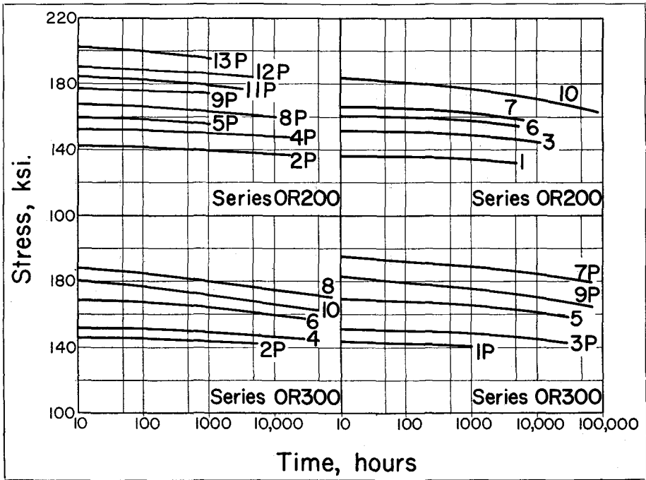
Fig. A.4—Measured Variation of Steel Stress with Time; Series OR200 and OR300.
