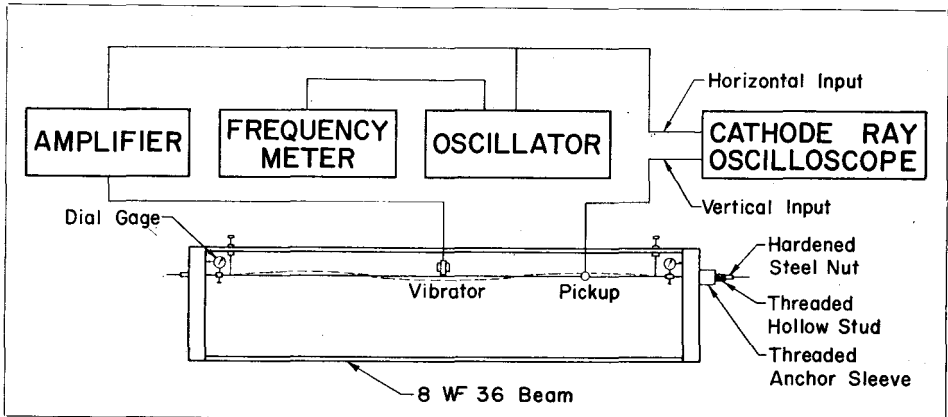
Fig. A.2—Schematic View of Test Setup.
