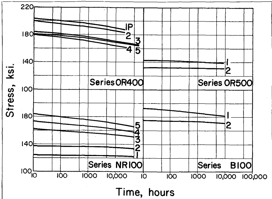
Fig. A.5—Measured Variation of Steel Stress with Time; Series OR400, NR100, and B100.
