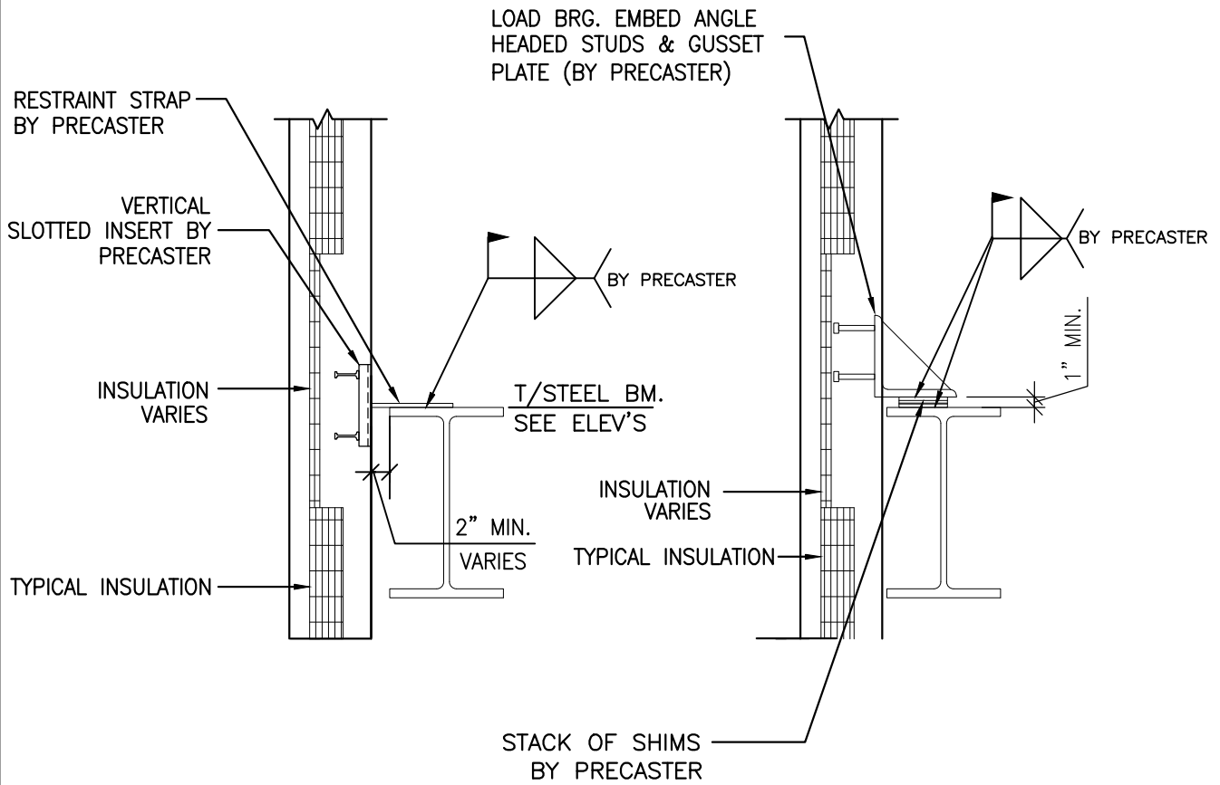
(A) PANEL TIE DETAIL
