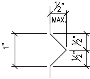
TYP. "V" GROOVE DETAIL
