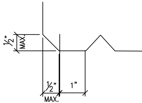
DRIP DETAIL
