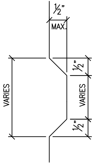
TYP. REVEAL DETAIL
