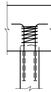
d) Hooked Dowels with Spiral
