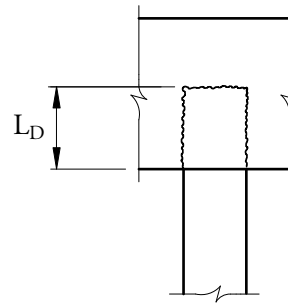
b) Pile Development with 1/4" Amplitude Roughening
