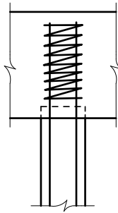
e) Exposed Strands with Spiral
