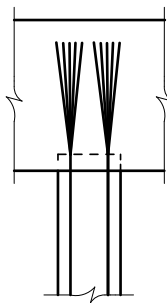
g) Exposed and "Broomed" Strands
