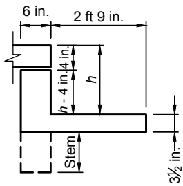
Single riser
