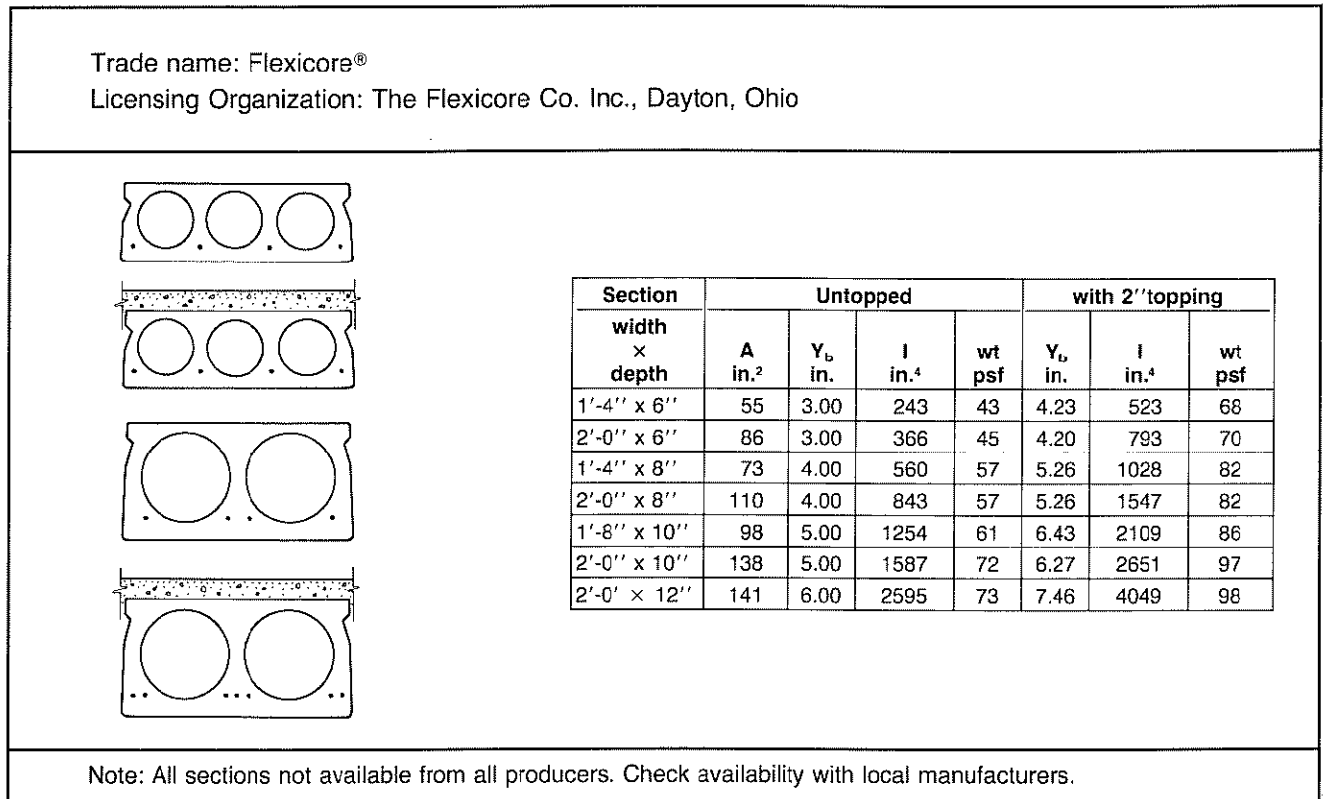
Fig. 2.4.3 Section properties — normal weight concrete
