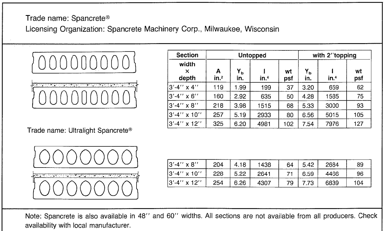
Fig. 2.4.4 Section properties — normal weight concrete
