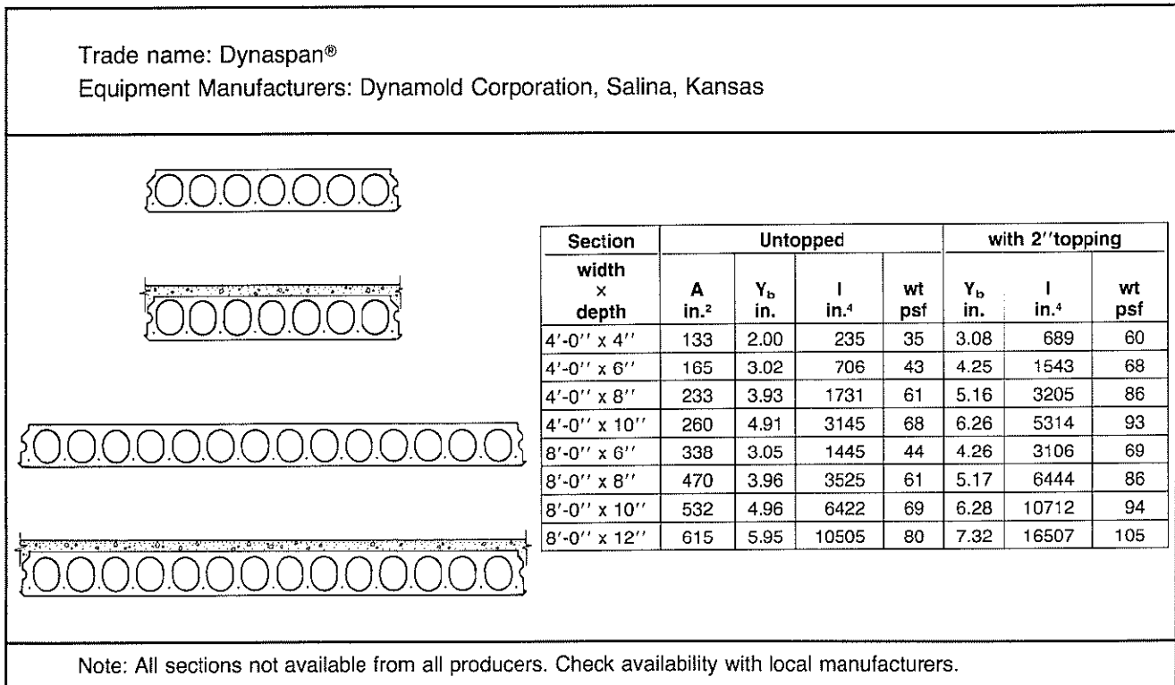
Fig. 2.4.2 Section properties — normal weight concrete
