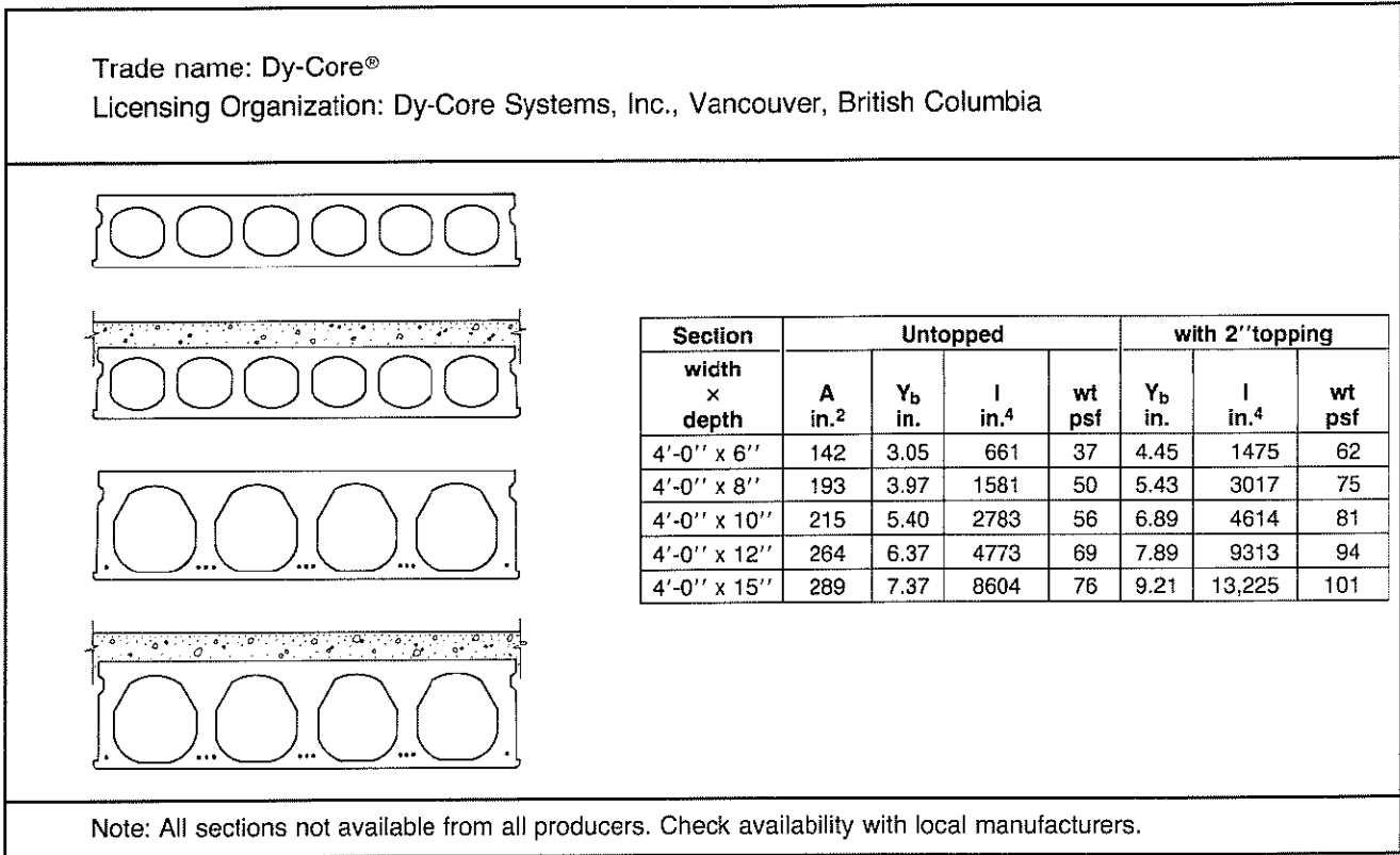
Fig. 2.4.2 Section properties — normal weight concrete
