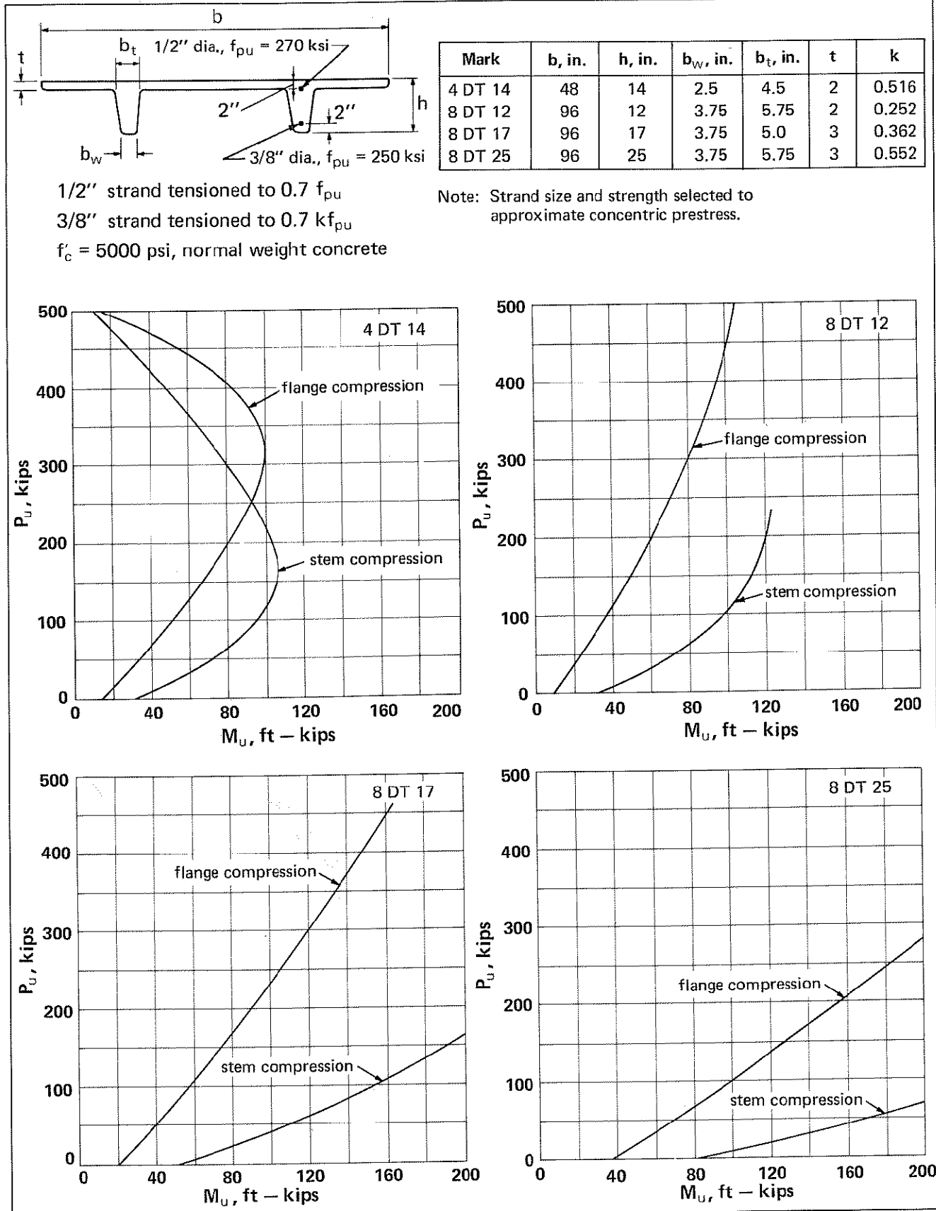
Fig. 3.6.1 Design (ultimate) capacity of prestressed concrete double-tee wall panels
