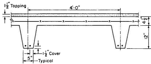
Fig. 8. Siliceous aggregate cast-in-place—restrained with 1 1/2" lightweight concrete topping.
