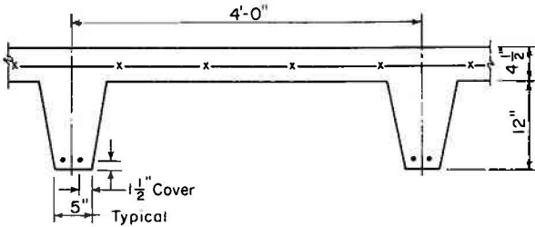
Fig. 7. Siliceous aggregate cast-in-place—restrained.
