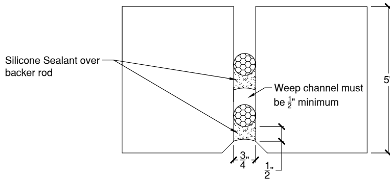
Detail 4A - Dual Sealant and Backer Rod (Control)
