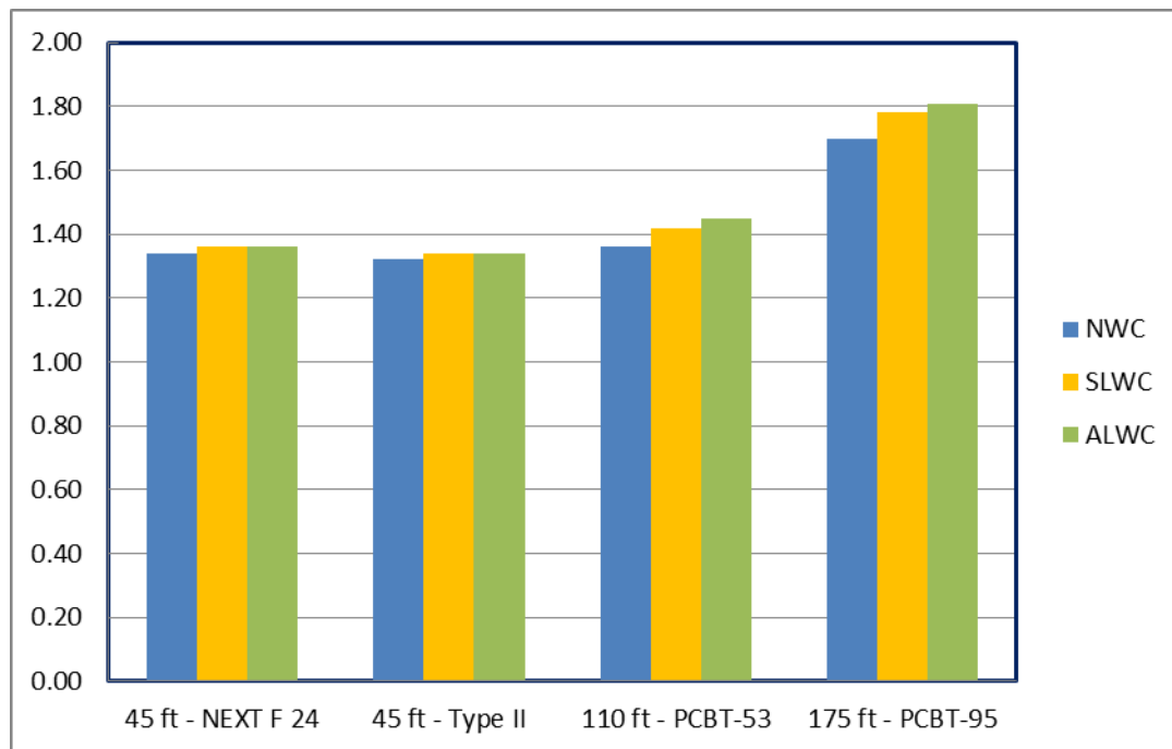
Fig. 7 Operating rating: Flexure
