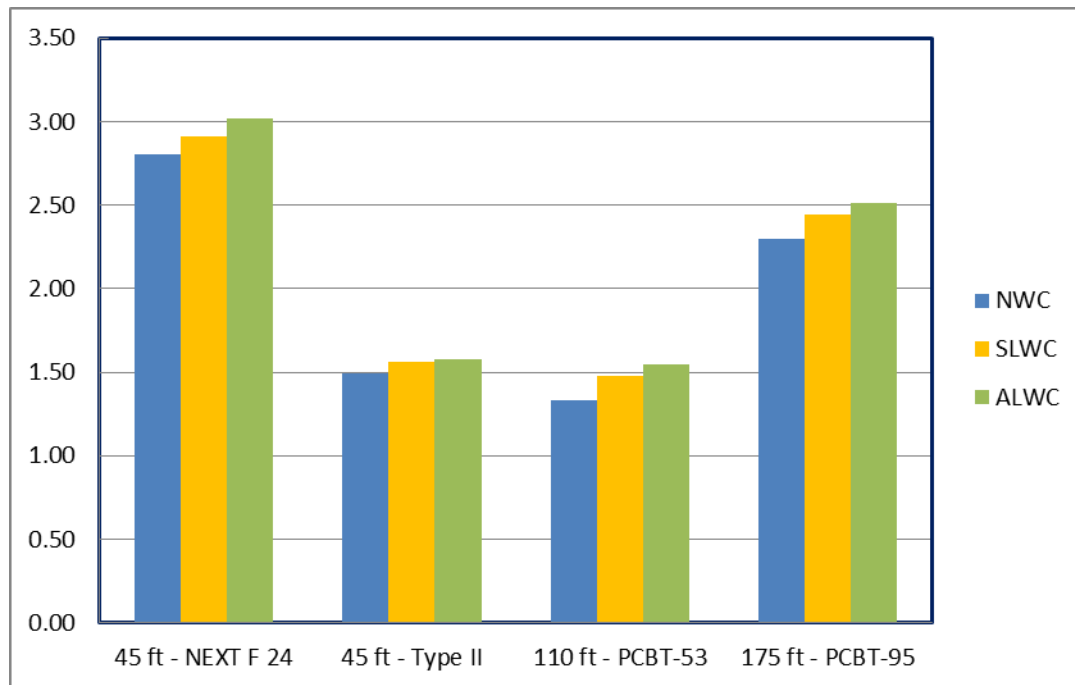
Fig. 8 Operating rating: Shear
