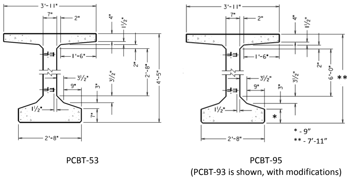
Fig. 2 Dimensions of VDOT standard girder sections used for medium and long span designs (from VDOT standard girder details 8 )
