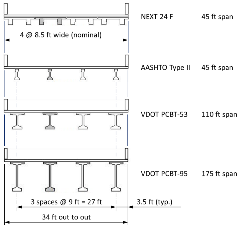
Fig. 1 Typical sections considered in study
