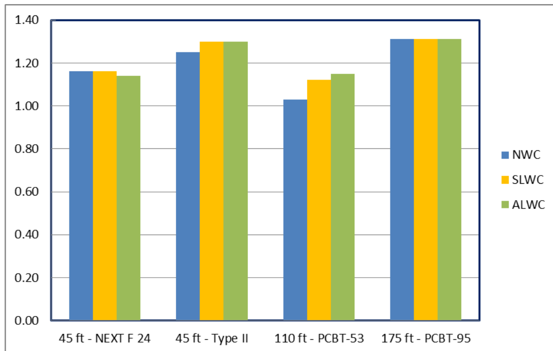
Fig. 3 Inventory rating: Service load – tensile stress
