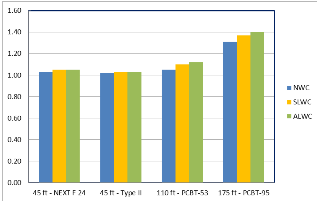
Fig. 5 Inventory rating: Strength – Flexure
