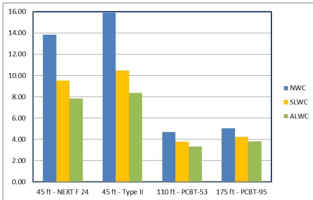
Fig. 4 Inventory rating: Service load – compression stress
