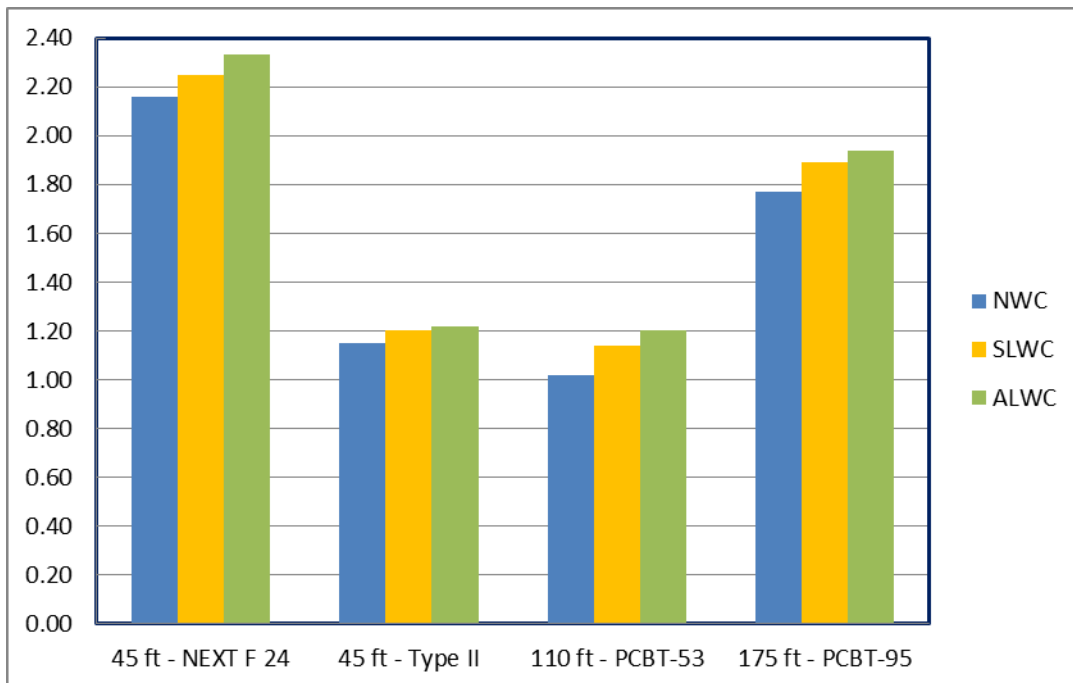
Fig. 6 Inventory rating: Strength – Shear
