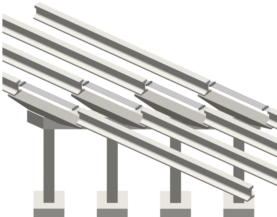
Fig. 1 Showing the pier section before placement of the pier blocks.
