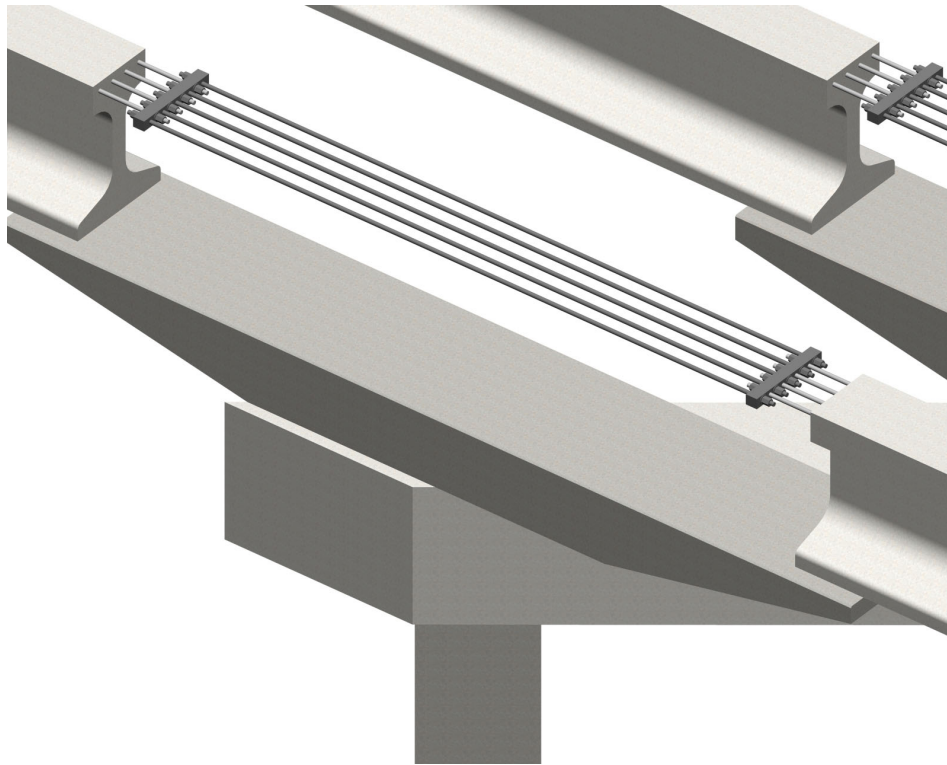
Fig. 2 Close-up view of the continuity connection
