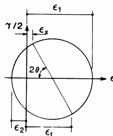
Fig. 1 Mohr's Circle for Strain
