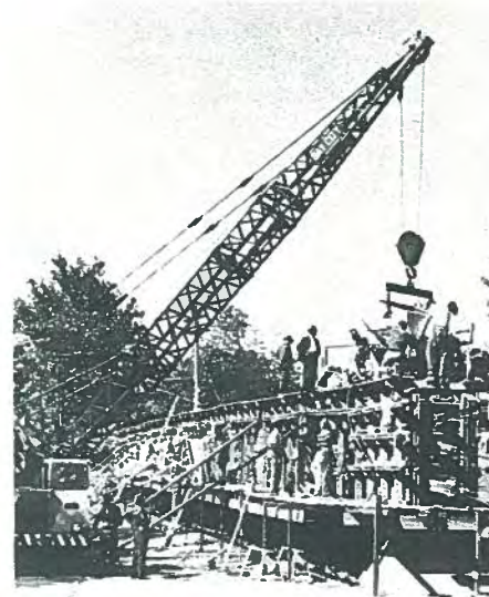
Fig. 3. Placing of concrete in Walnut Lane test girder.
