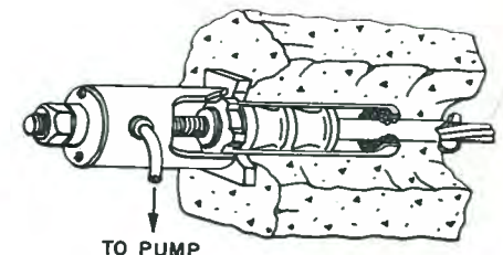
Fig. 9b. Typical Roebing anchorage (after stressing).
